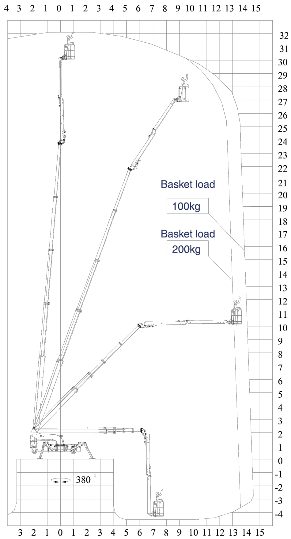
FS320 FALCON SPIDER REACH DIAGRAM
