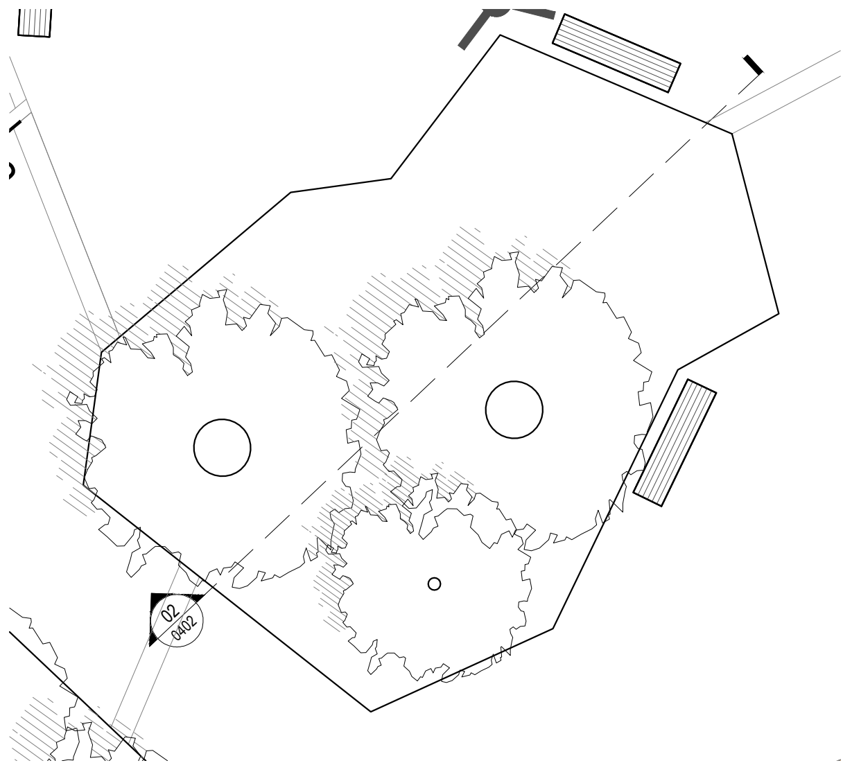
01 0402 KEY PLAN Scale 1: 100 @A1
