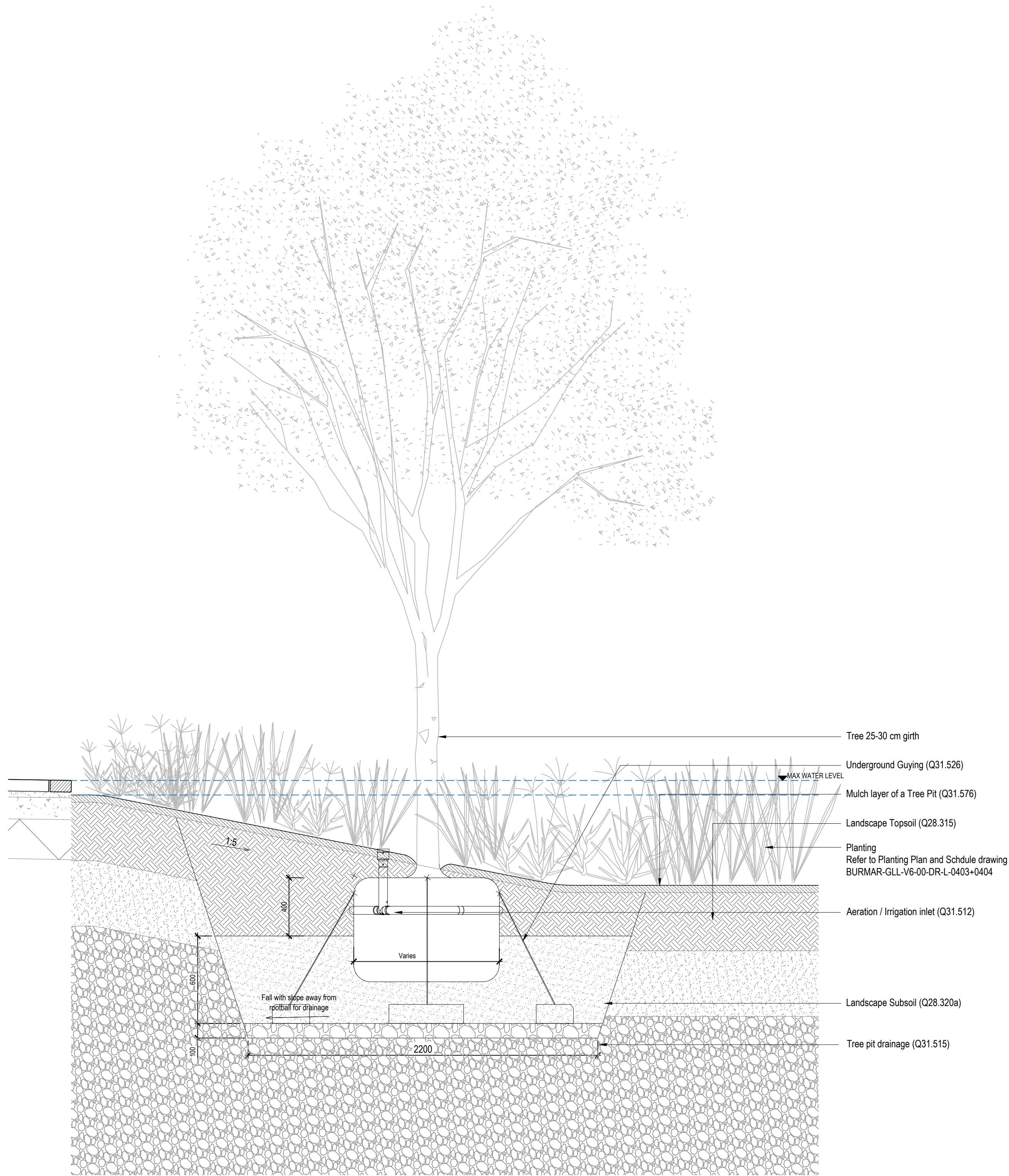
02 0401 TYPICAL RAINGARDEN TREE PIT DETAIL Scale 1: 20 @A1
