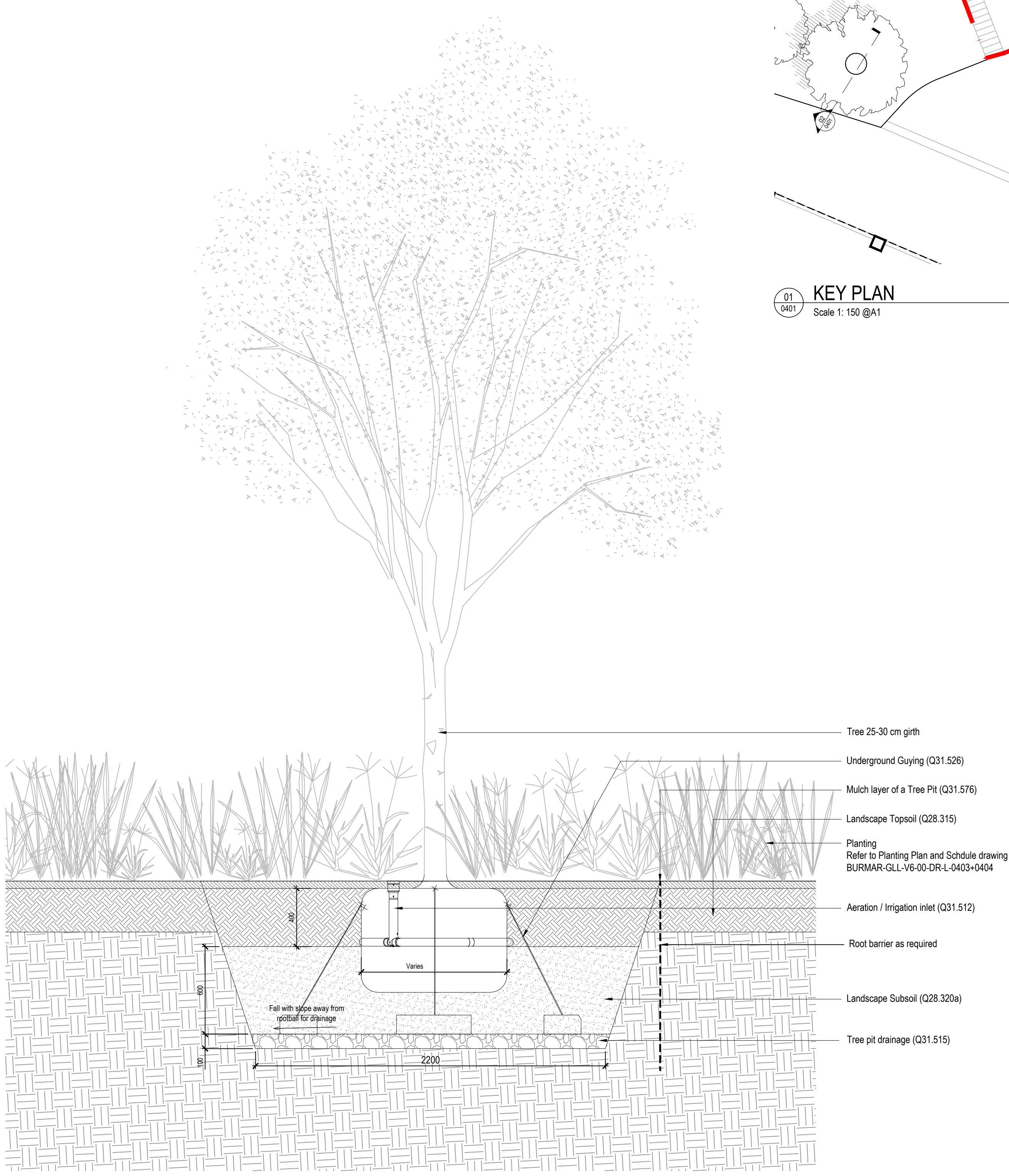
03 0401 TYPICAL PLANTING TREE PIT DETAIL Scale 1: 20 @A1
