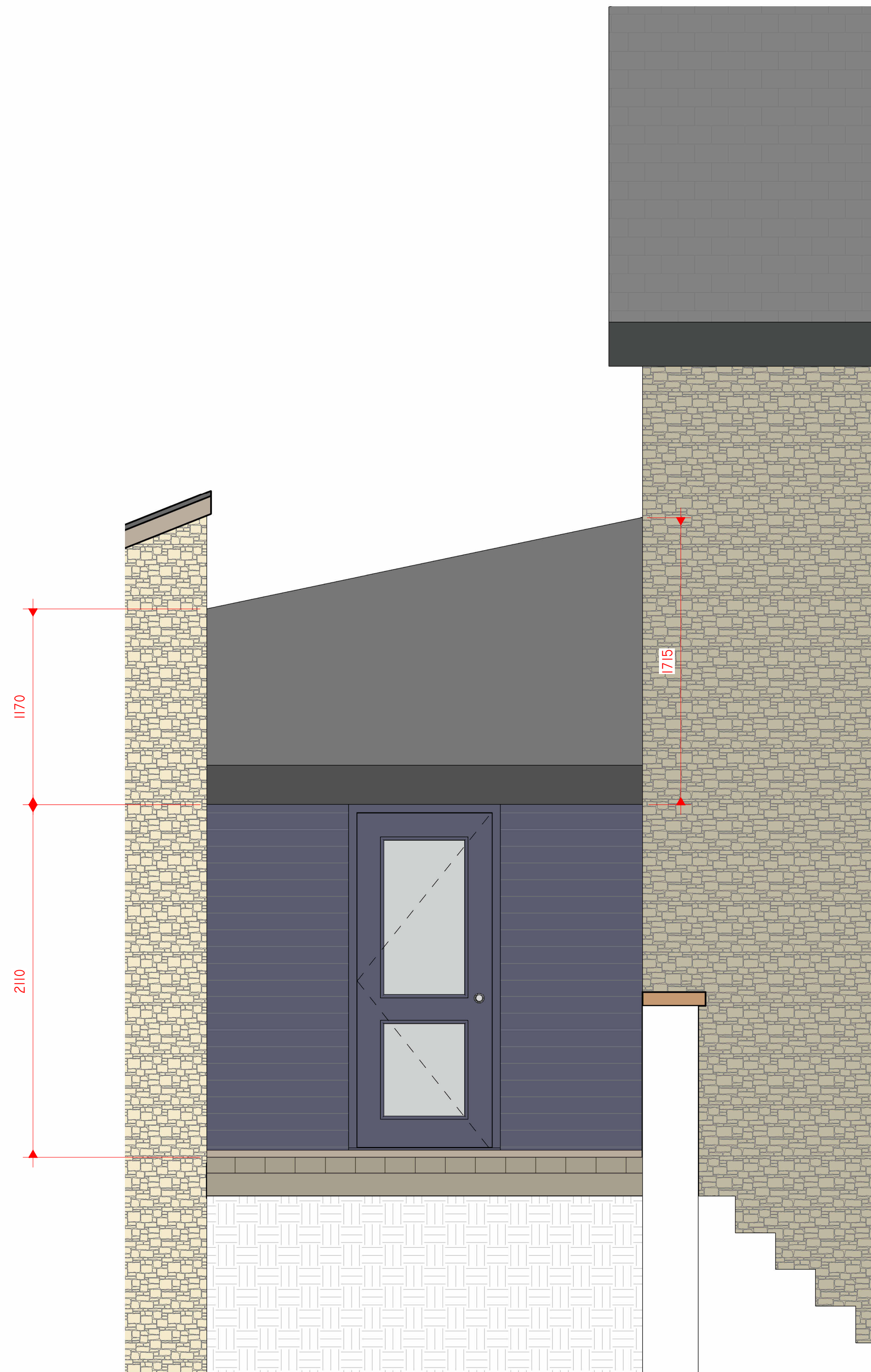
2 EXISTING PORCH ELEVATION 1 : 20
