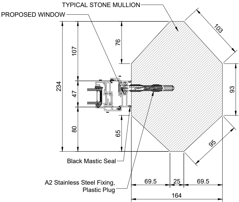
TYPICAL SECTION Scale 1:4
