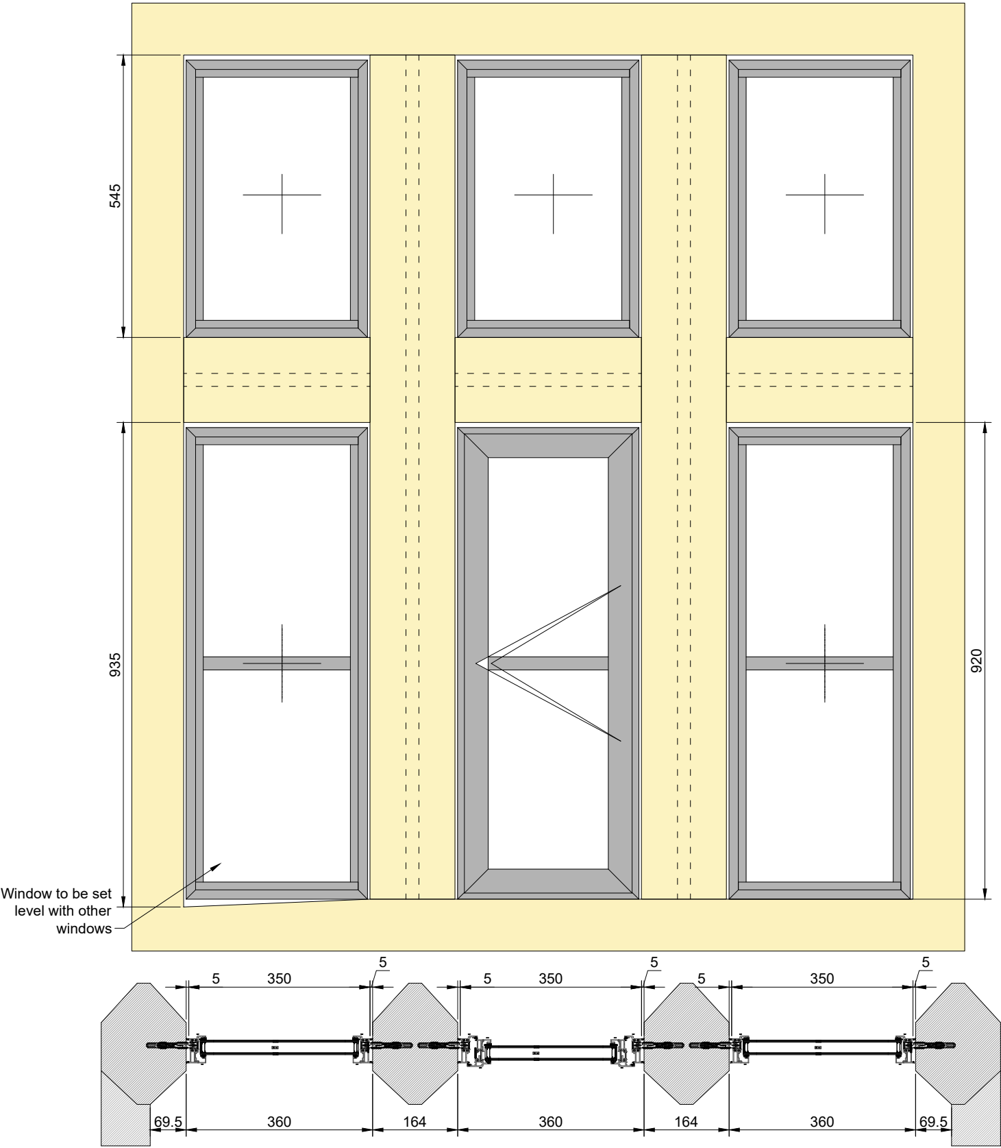
Front Elevation 1st Floor Right Side
