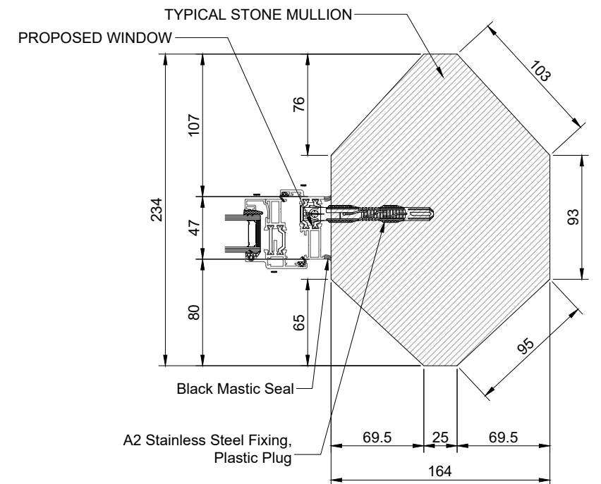
TYPICAL SECTION Scale 1:4
