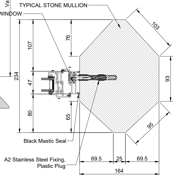
TYPICAL SECTION Scale 1:4
