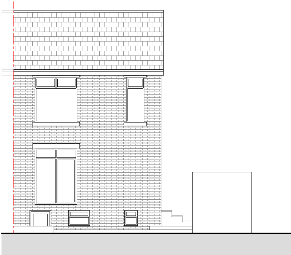
EXISTING REAR ELEVATION 1:100 @ A3
