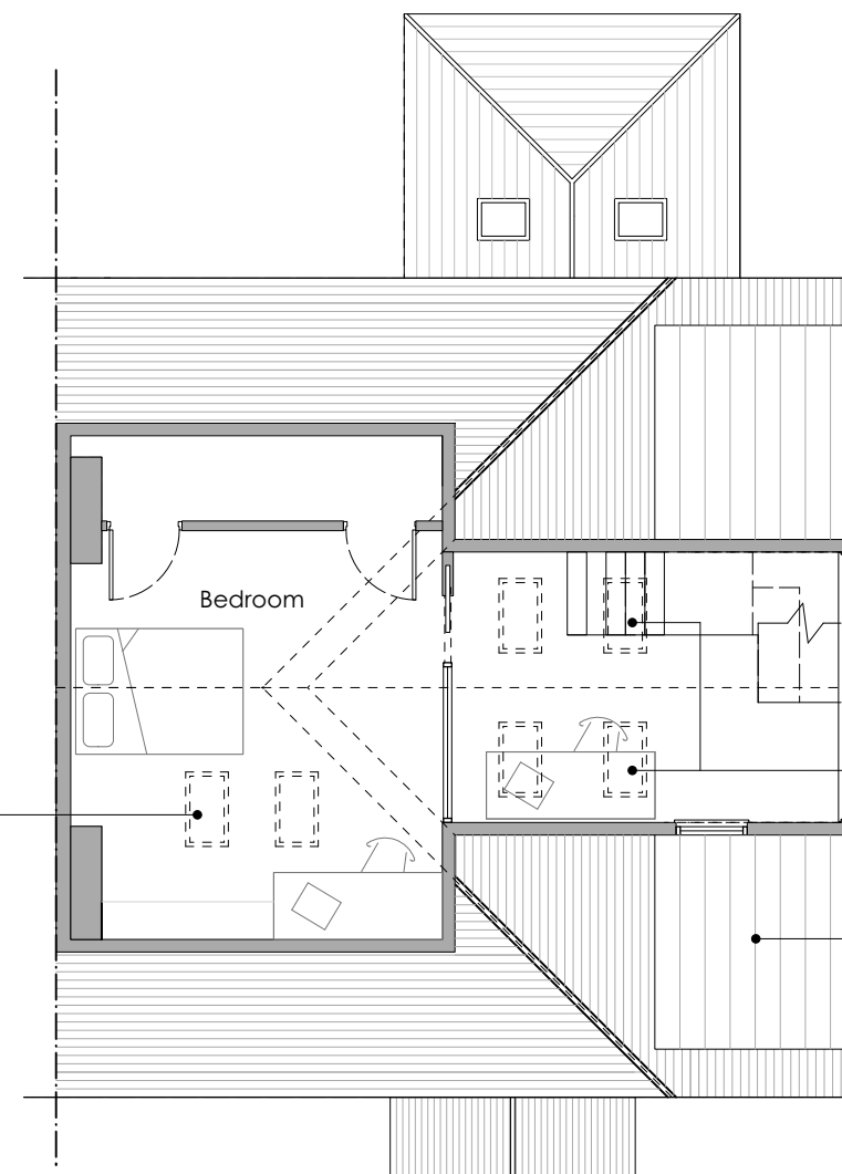
Proposed Second floor plan 1:100
