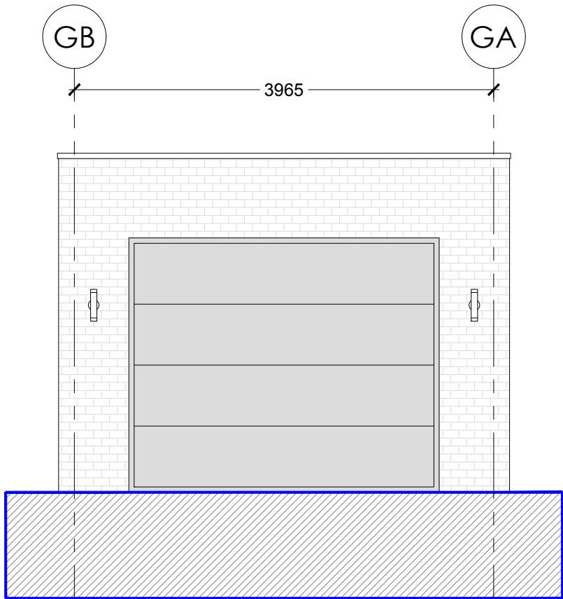
DETACHED GARAGE, FRONT ELEVATION 1:50
