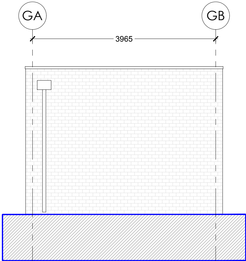
DETACHED GARAGE, REAR ELEVATION 1:50
