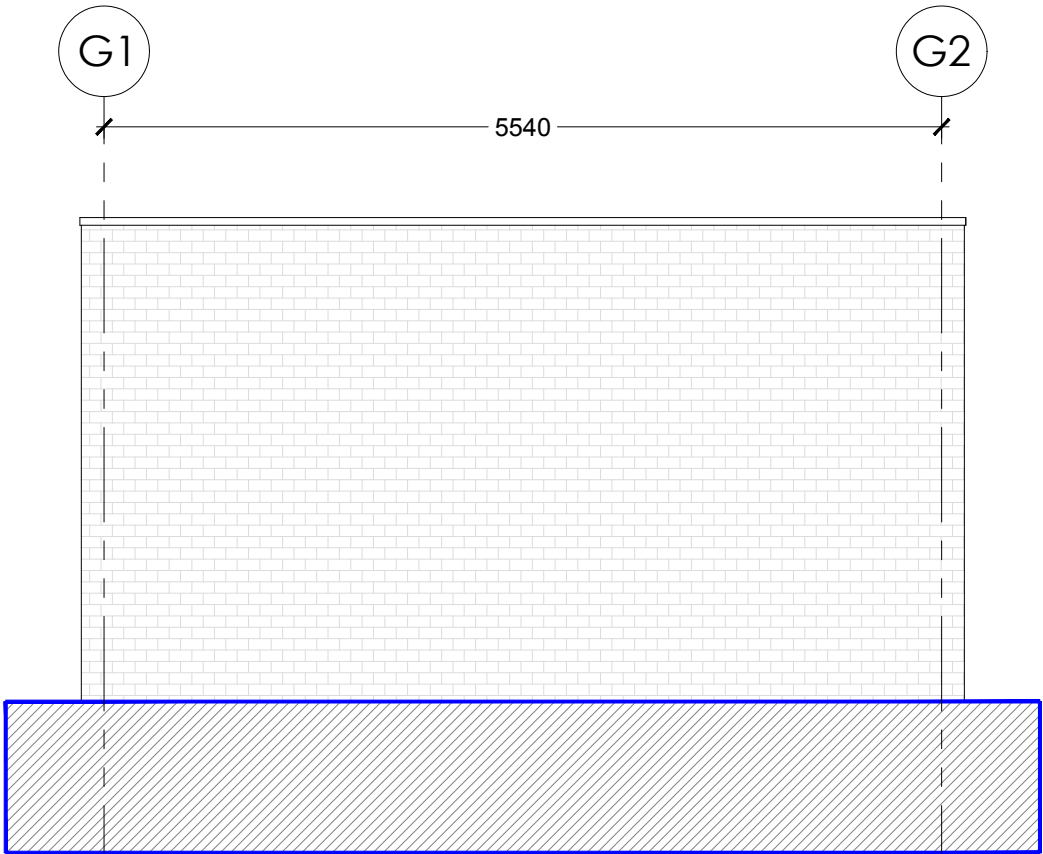
DETACHED GARAGE, SIDE ELEVATION 1:50
