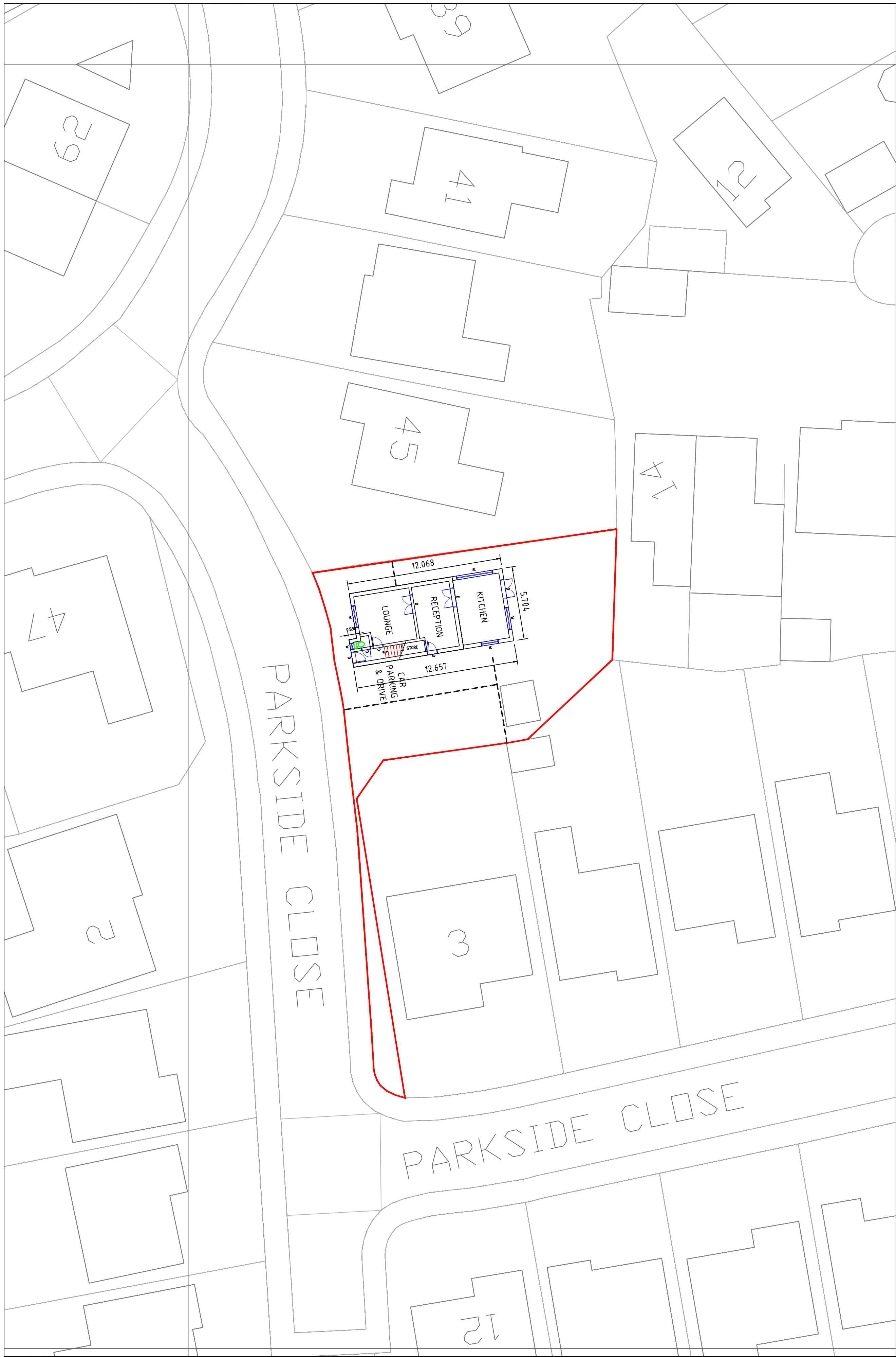
EXISTING SITE LAYOUT
