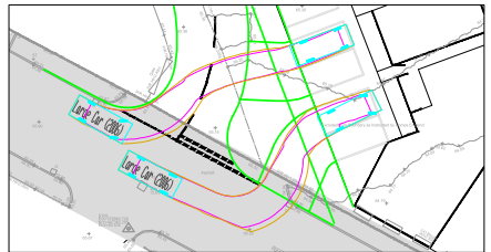
SWEPT PATH ANALYSIS - LARGE CAR
