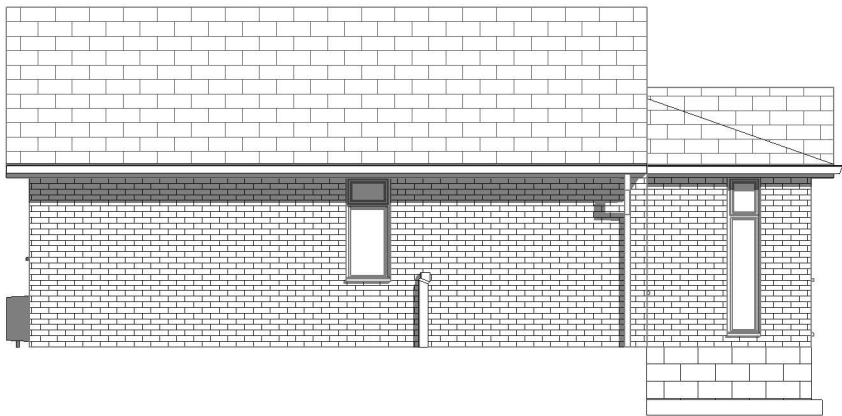
3 Side Elevation 1 : 100
