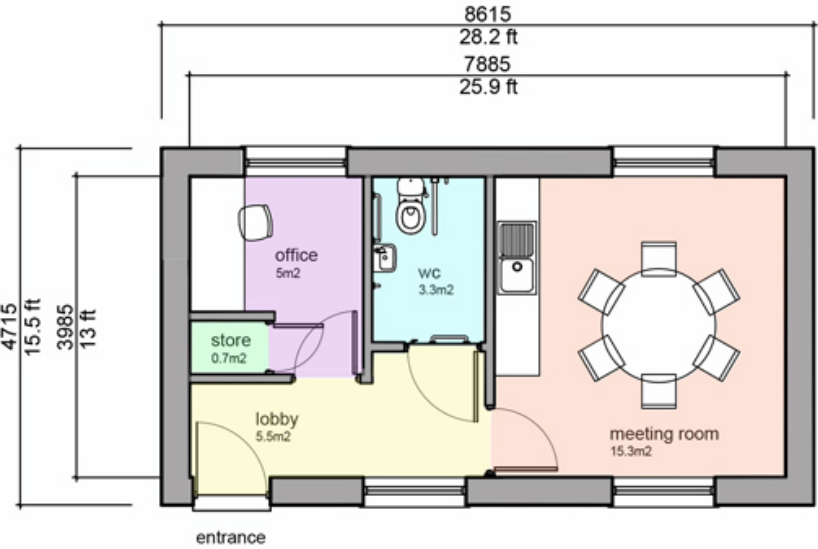
management block plan 31.4 m2
