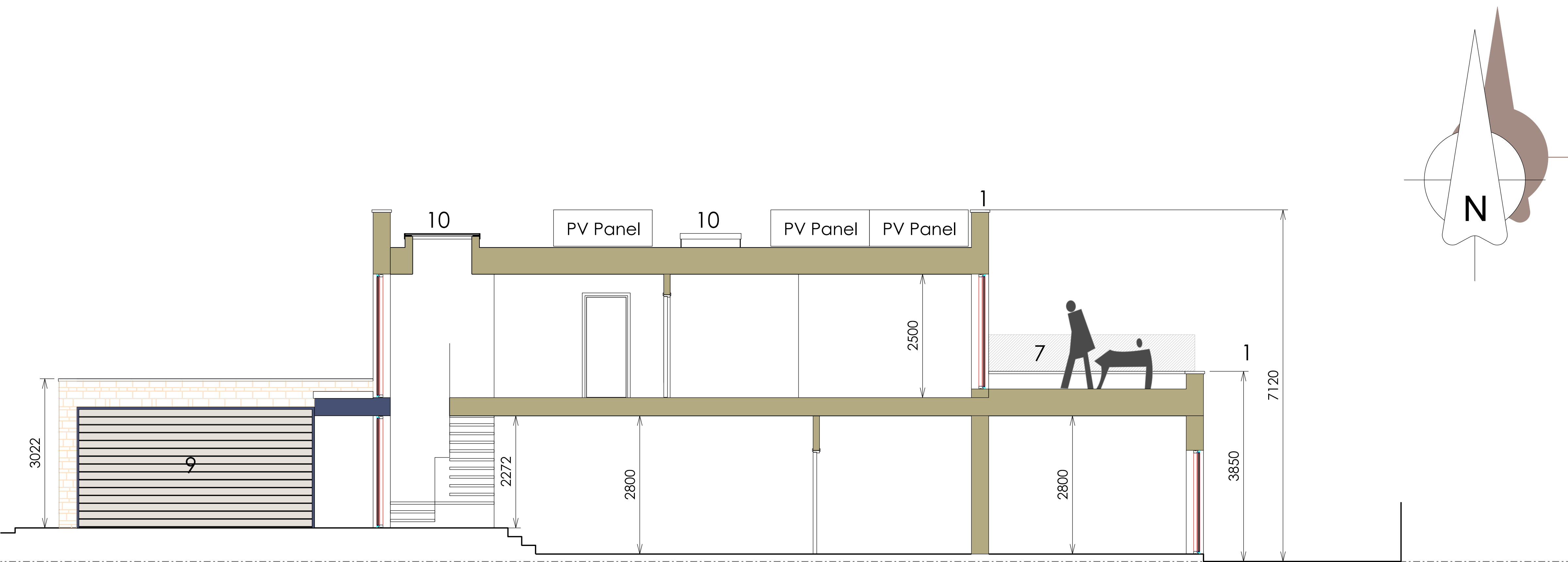
PROPOSED SECTION A - A 1:50
