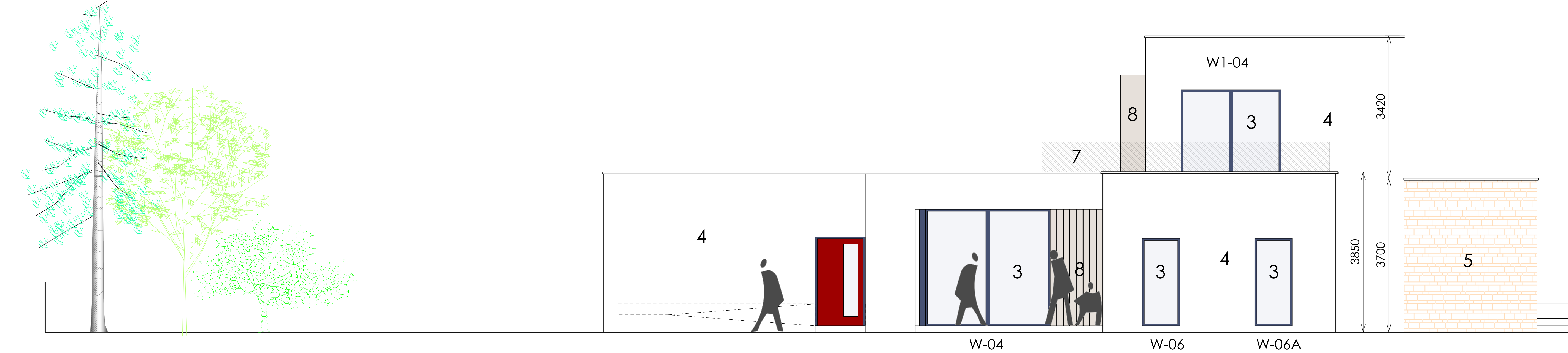
PROPOSED EAST ELEVATION
