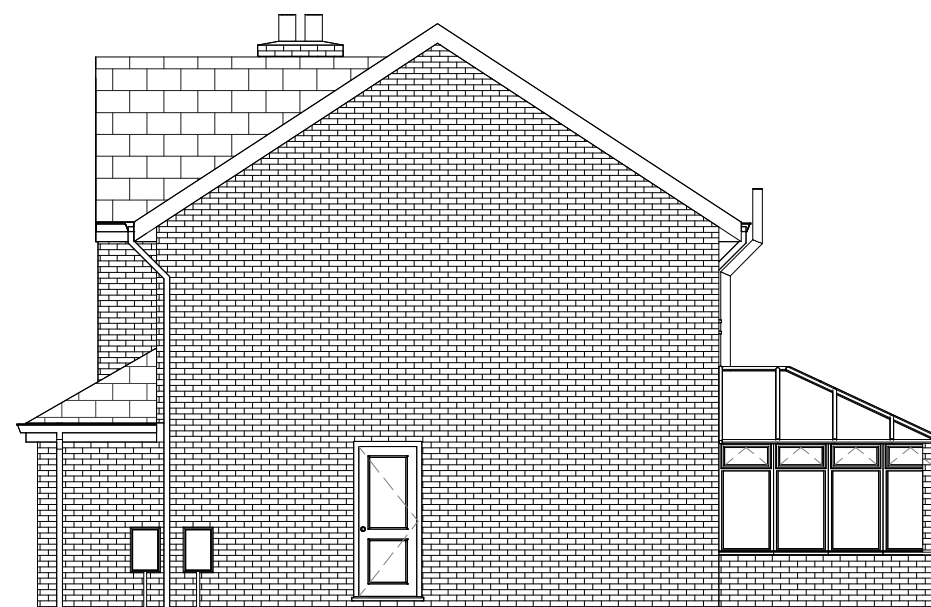
2 Garage Elevation 1 : 100
