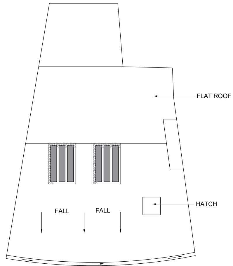
ROOF PLAN
