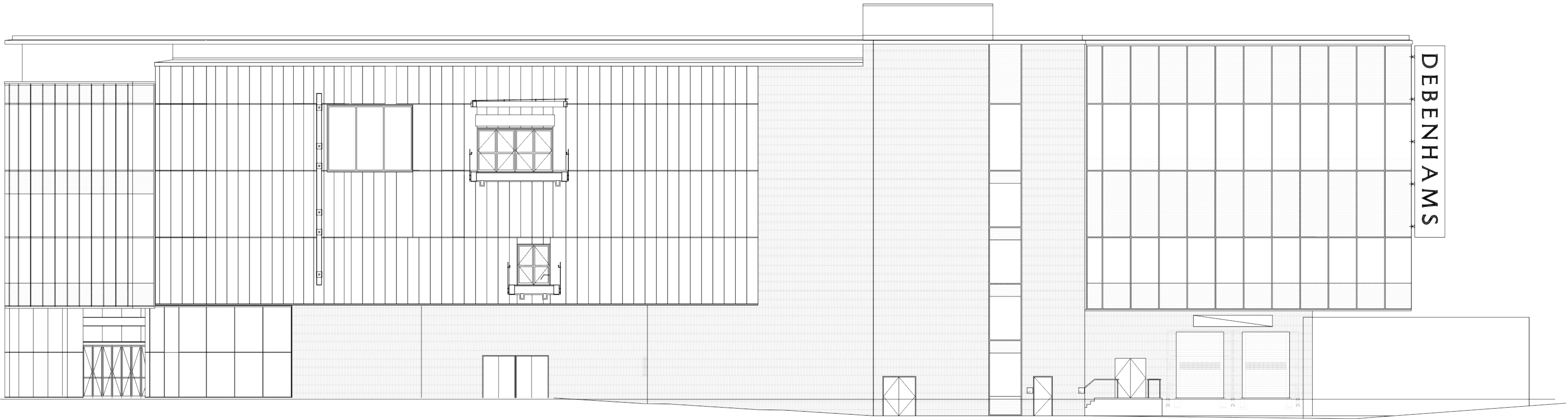
EXISTING 1:100 scale
