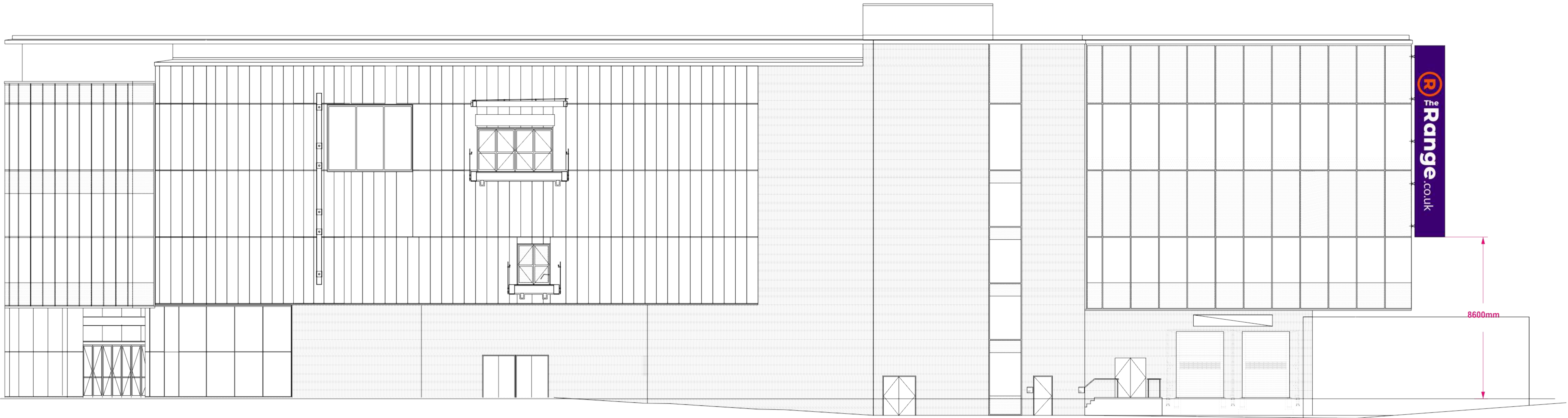
PROPOSED 1:100 scale
