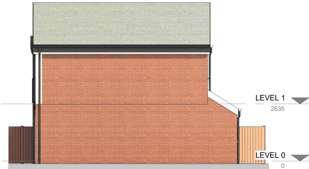
4. Left Side - Existing 1 : 100
