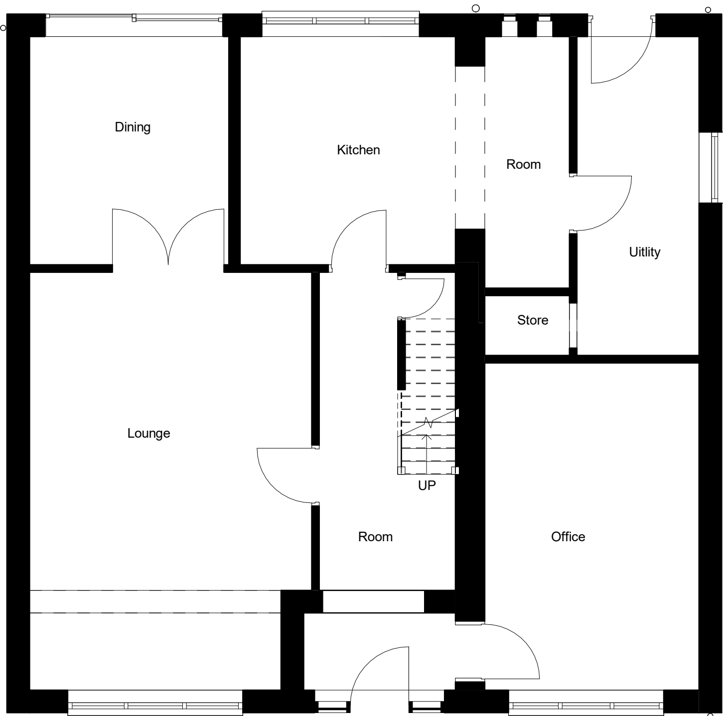
1. Level 0 - GA Existing 1 : 50
