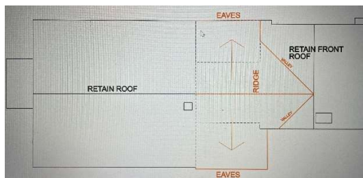
proposed roof plan (new in orange)
