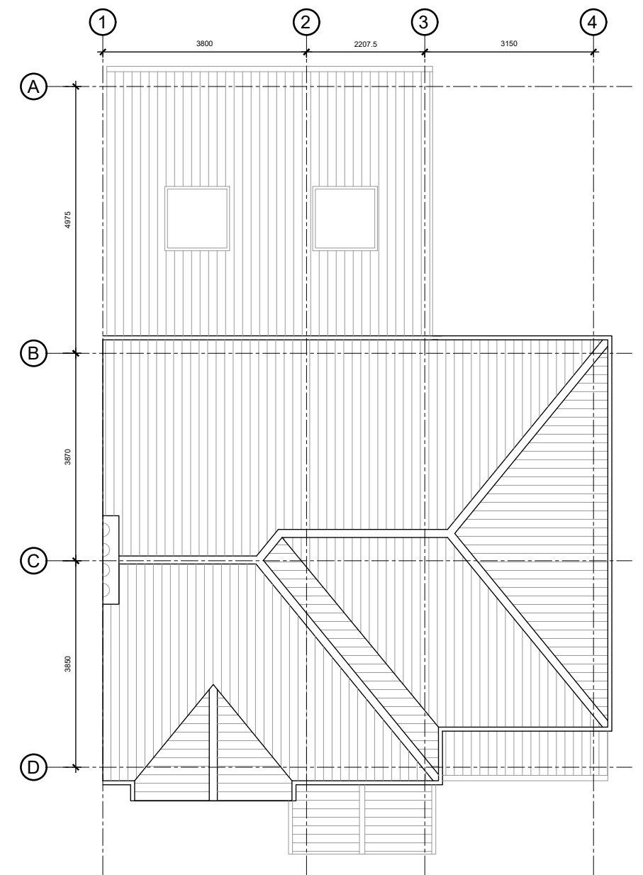
PROPOSED ROOF
