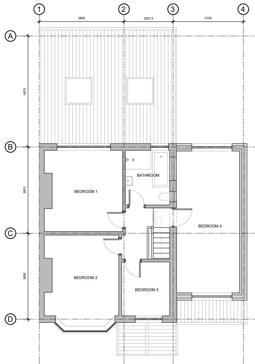
PROPOSED FIRST FLOOR
