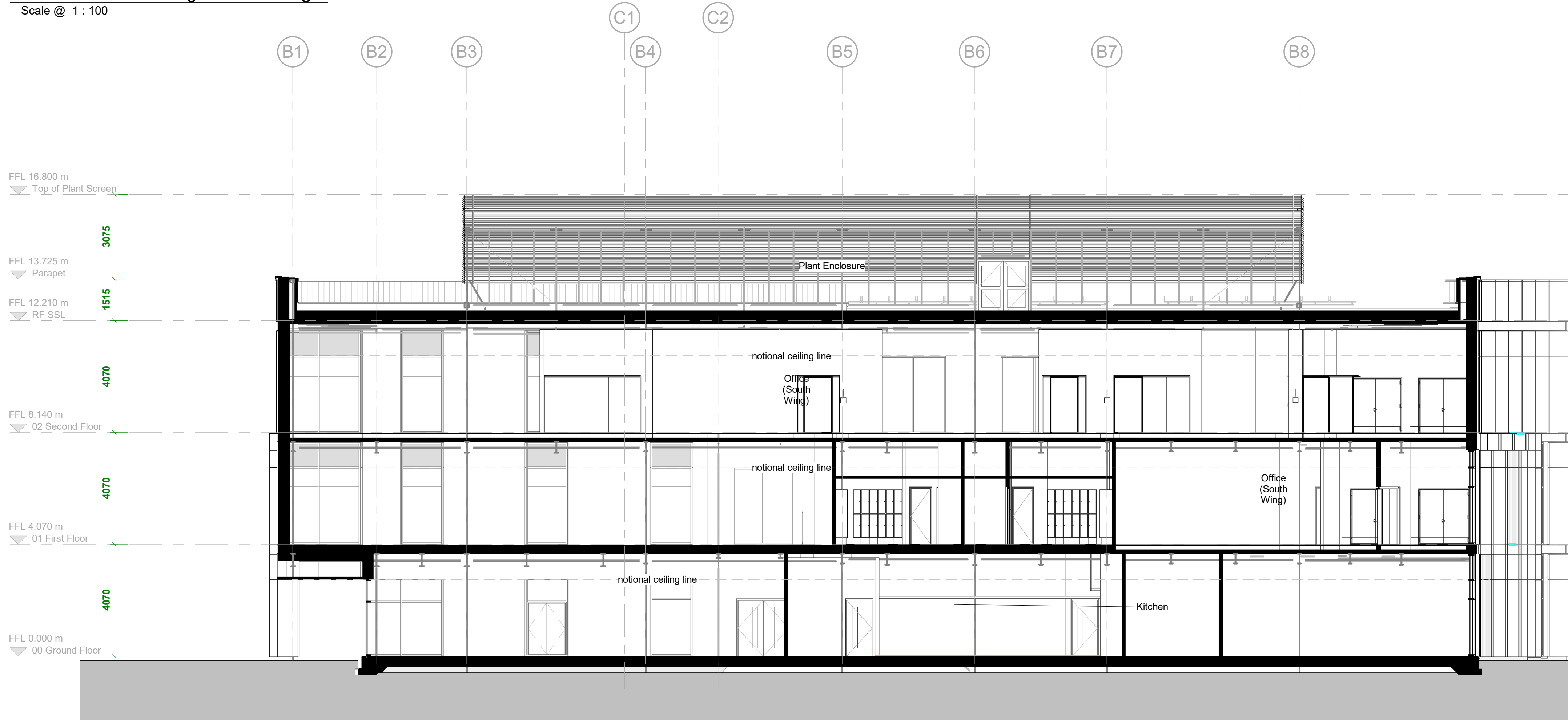
Section BB - Through South Wing Scale @ 1 : 100
