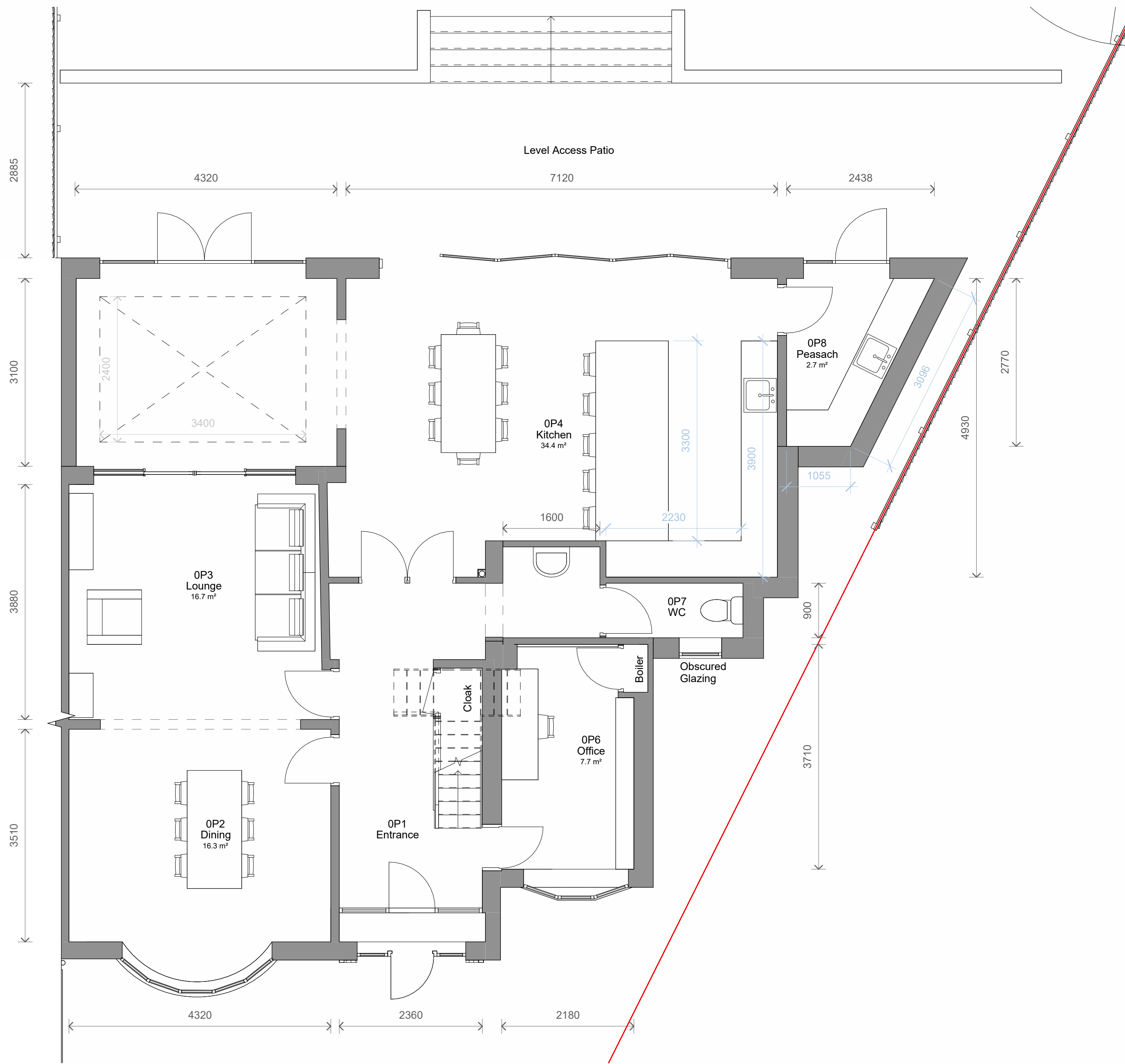
1 Level 0 - Proposed 1 : 50
