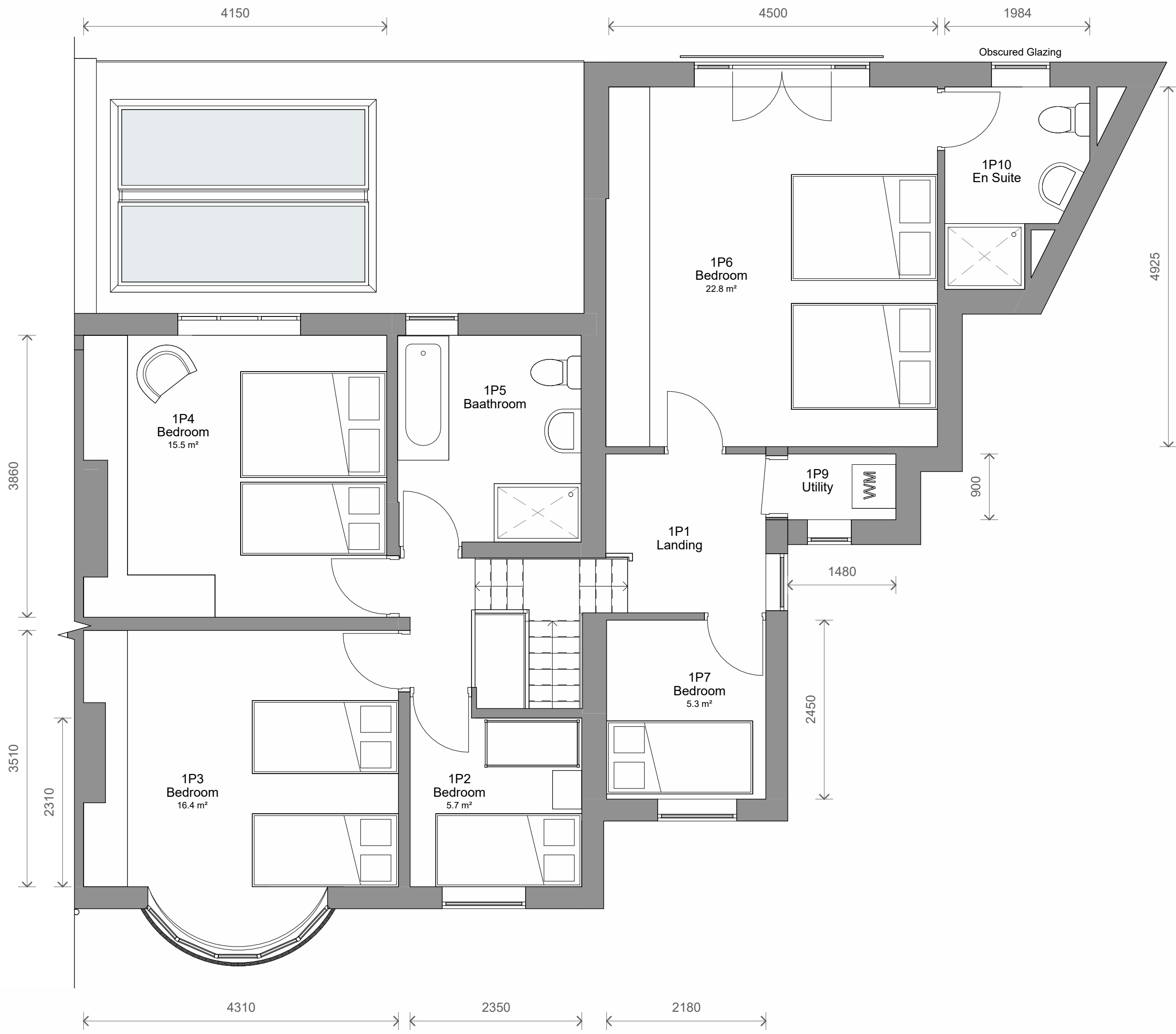
2 Level 1 - Proposed 1 : 50
