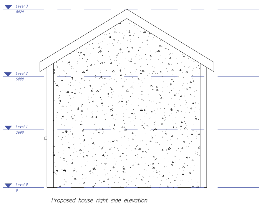
Proposed house right side elevation
