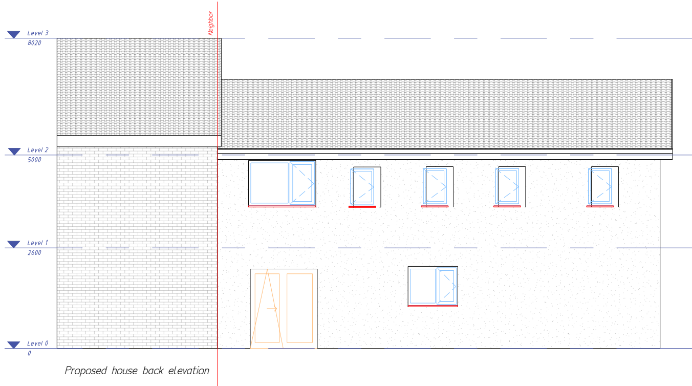
Proposed house back elevation
