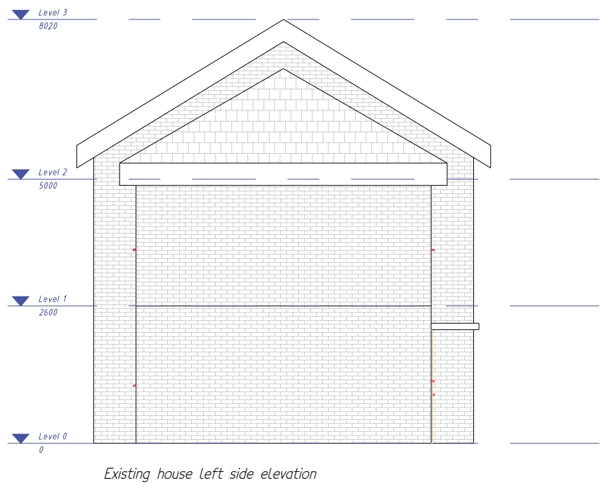
Existing house left side elevation
