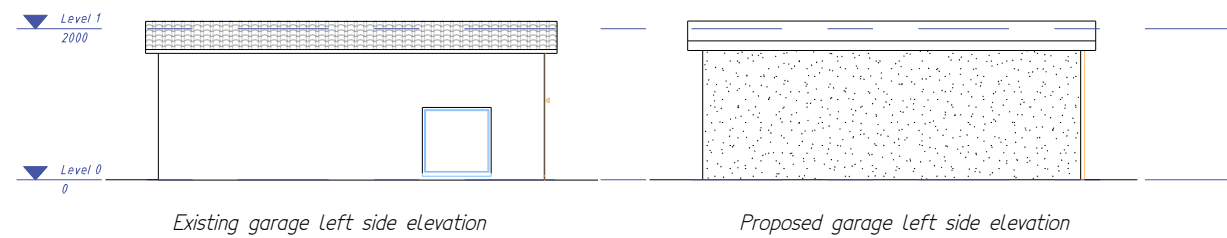
Existing garage left side elevation
