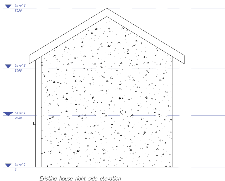
Existing house right side elevation
