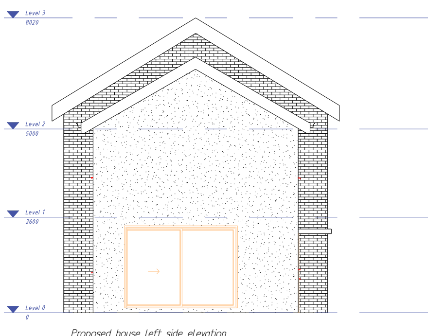
Proposed house left side elevation
