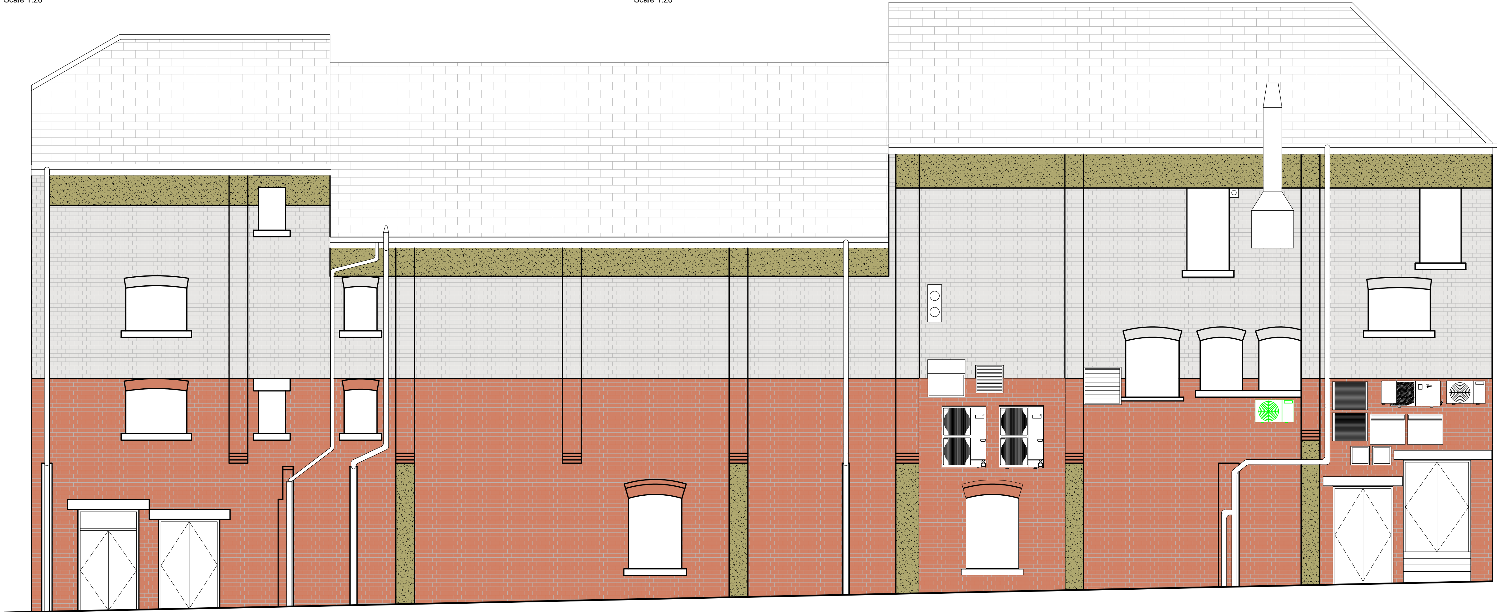
EXISTING ELEVATION B Scale 1:20
