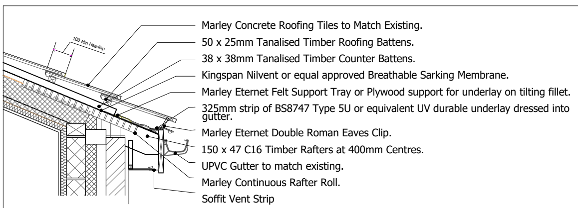
Typical wall/eaves details
