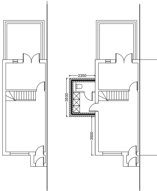
Existing – Proposed Floor Plans
