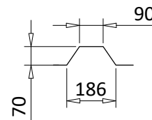
Male Recess
