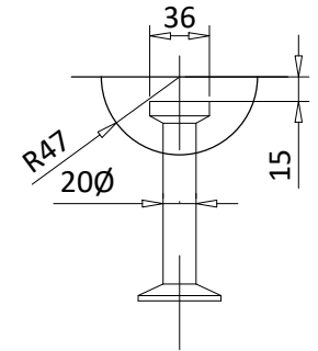
Pin Detail
