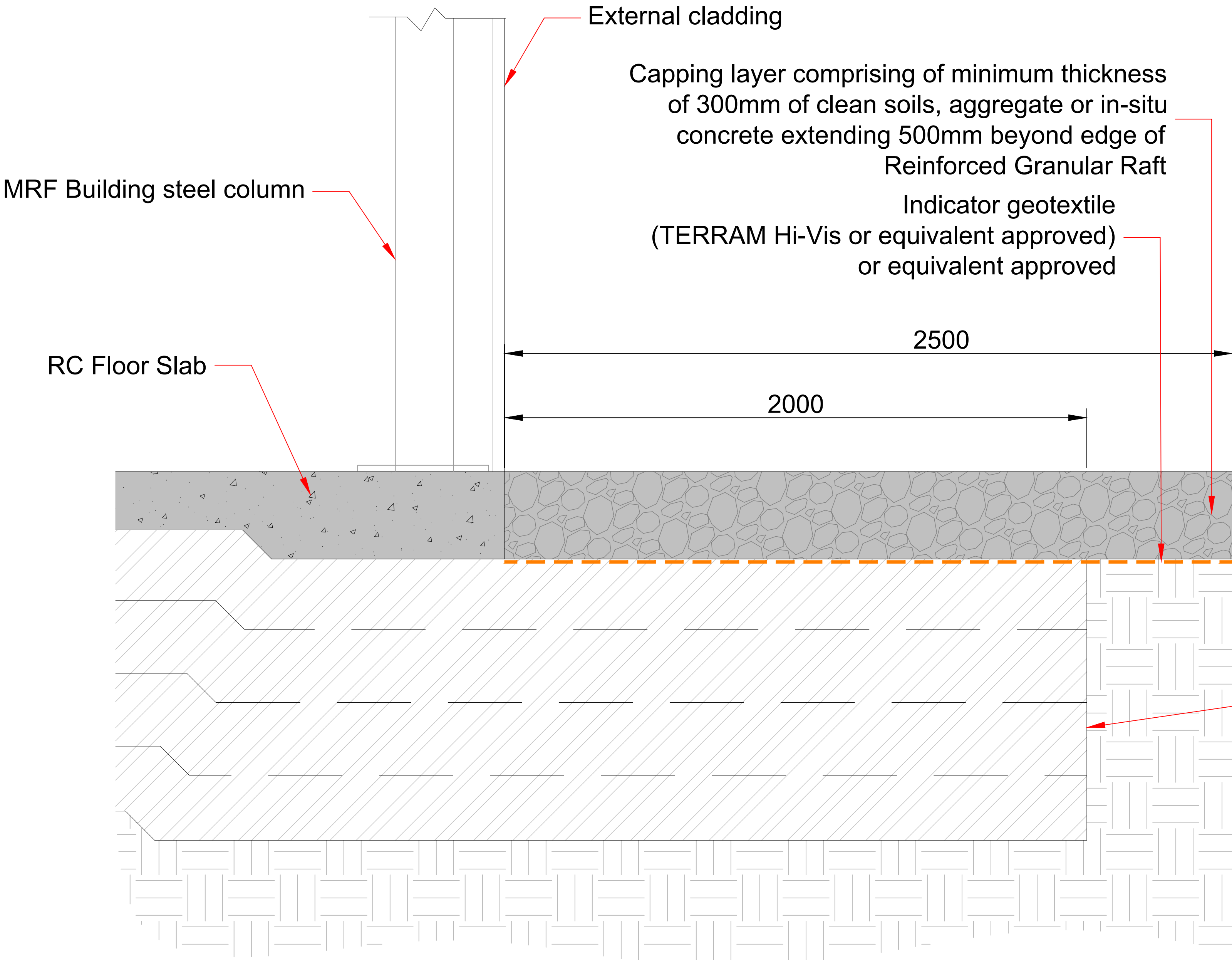
Capping Detail Scale 1:10
