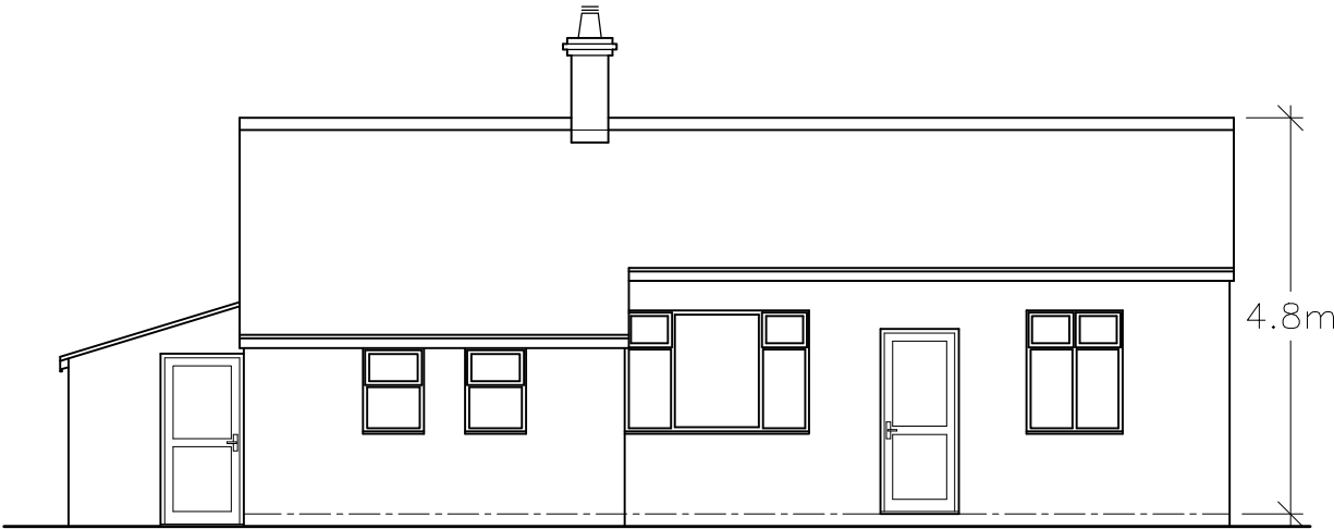
EXISTING SOUTH ELEVATION 1:100 scale
