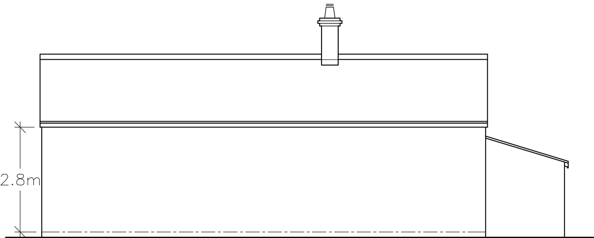
EXISTING NORTH ELEVATION 1:100 scale
