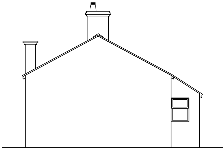
EXISTING WEST ELEVATION 1:100 scale
