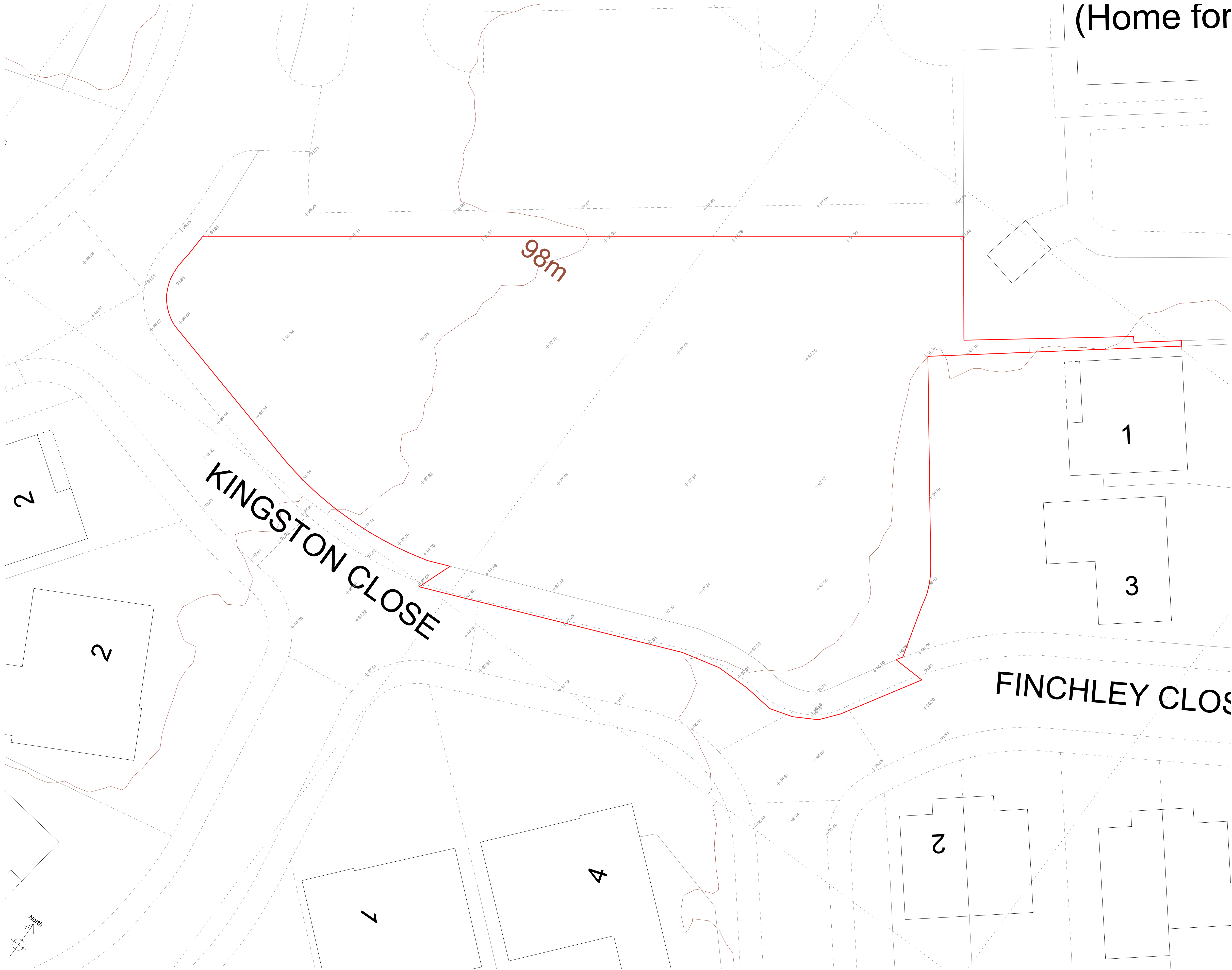
Existing Site Topographical Plan 1:150
