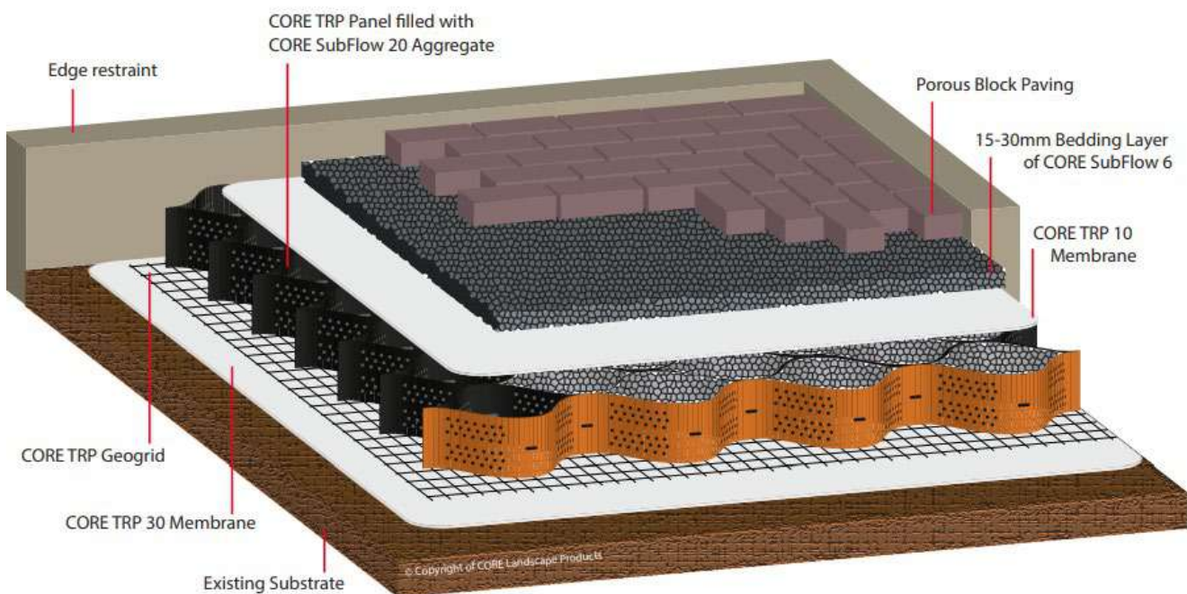
Figure 6. An example of a cellular confinement system with a block paving finishing course courtesy Core LP (for more details visit https://www.corelp.co.uk/core-tree-root-protection/ )
