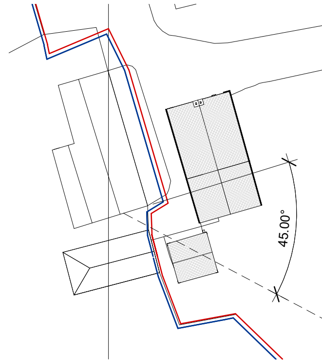
PLAN - 45 degree rule
