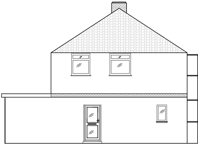
EXISTING LEFT ELEVATION
