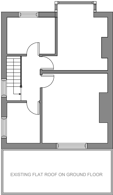
EXISTING 1ST FLOOR PLAN
