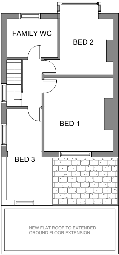
PROPOSED 1ST FLOOR PLAN
