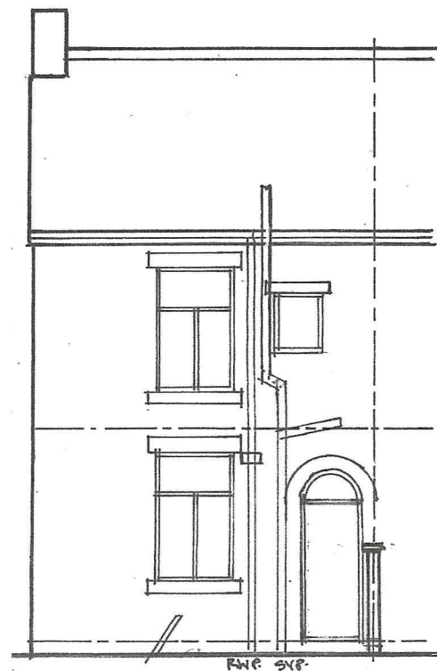
REAR ELEVATION
