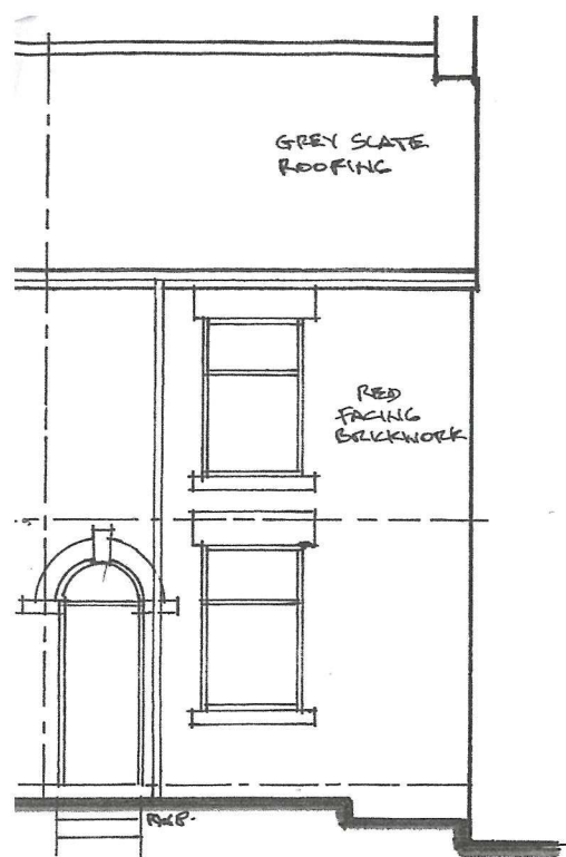
FRONT ELEVATION. 1:100
