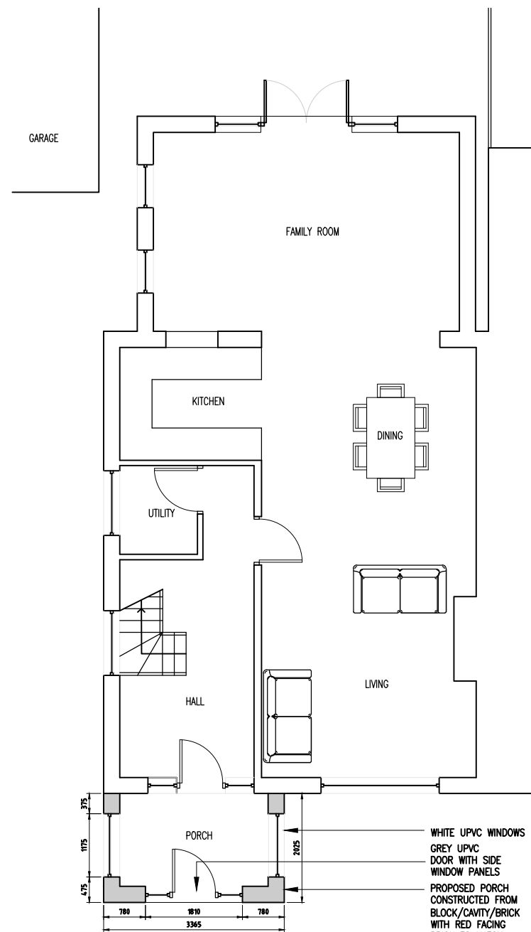
PROPOSED GROUND FLOOR LAYOUT 1:100 @ A3
