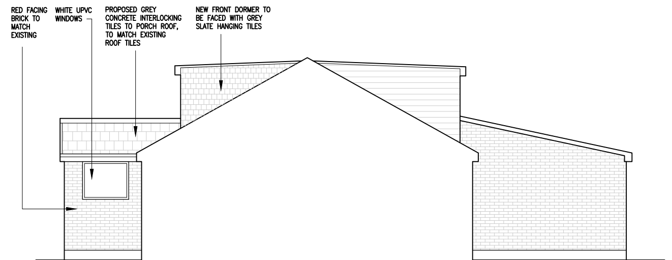
PROPOSED SIDE ELEVATION FROM NO.14 1:100 @ A3
