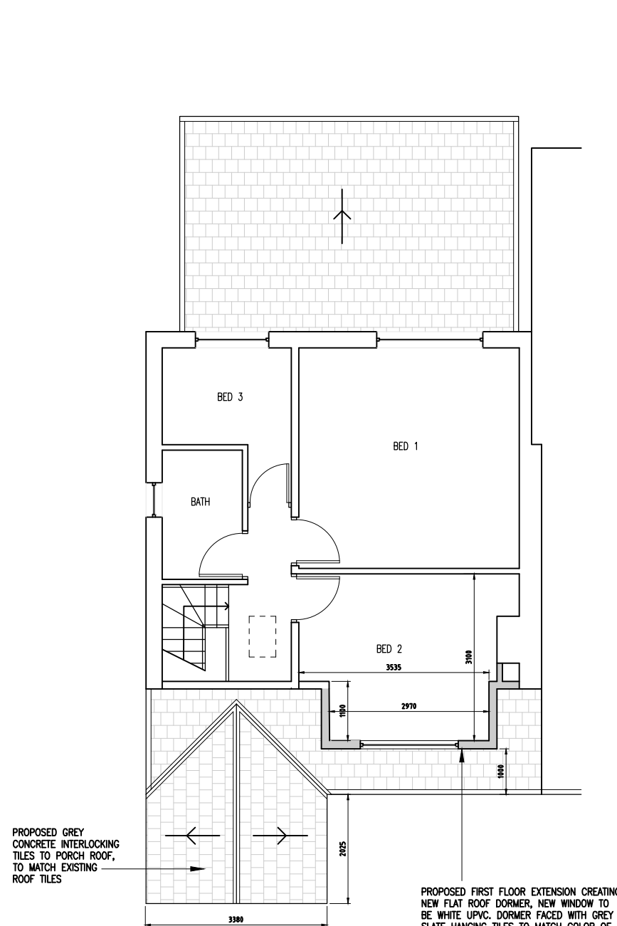
PROPOSED FIRST FLOOR LAYOUT 1:100 @ A3
