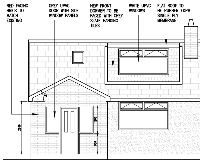
PROPOSED FRONT ELEVATION 1:100 @ A3
