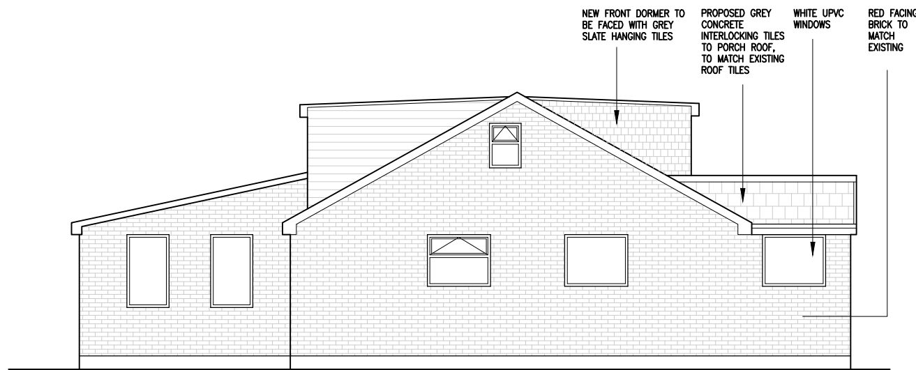
PROPOSED SIDE ELEVATION 1:100 @ A3
