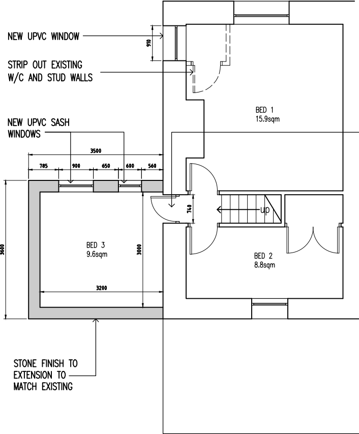
PROPOSED FIRST FLOOR PLAN 1:100 @ A3
