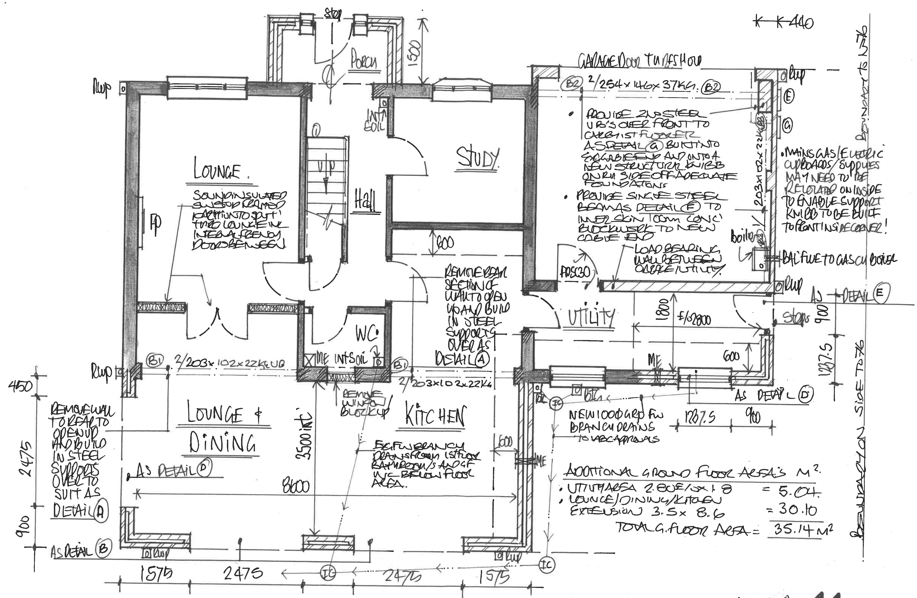
1:50 PROPOSED "GROUND FLOOR" PLAN
