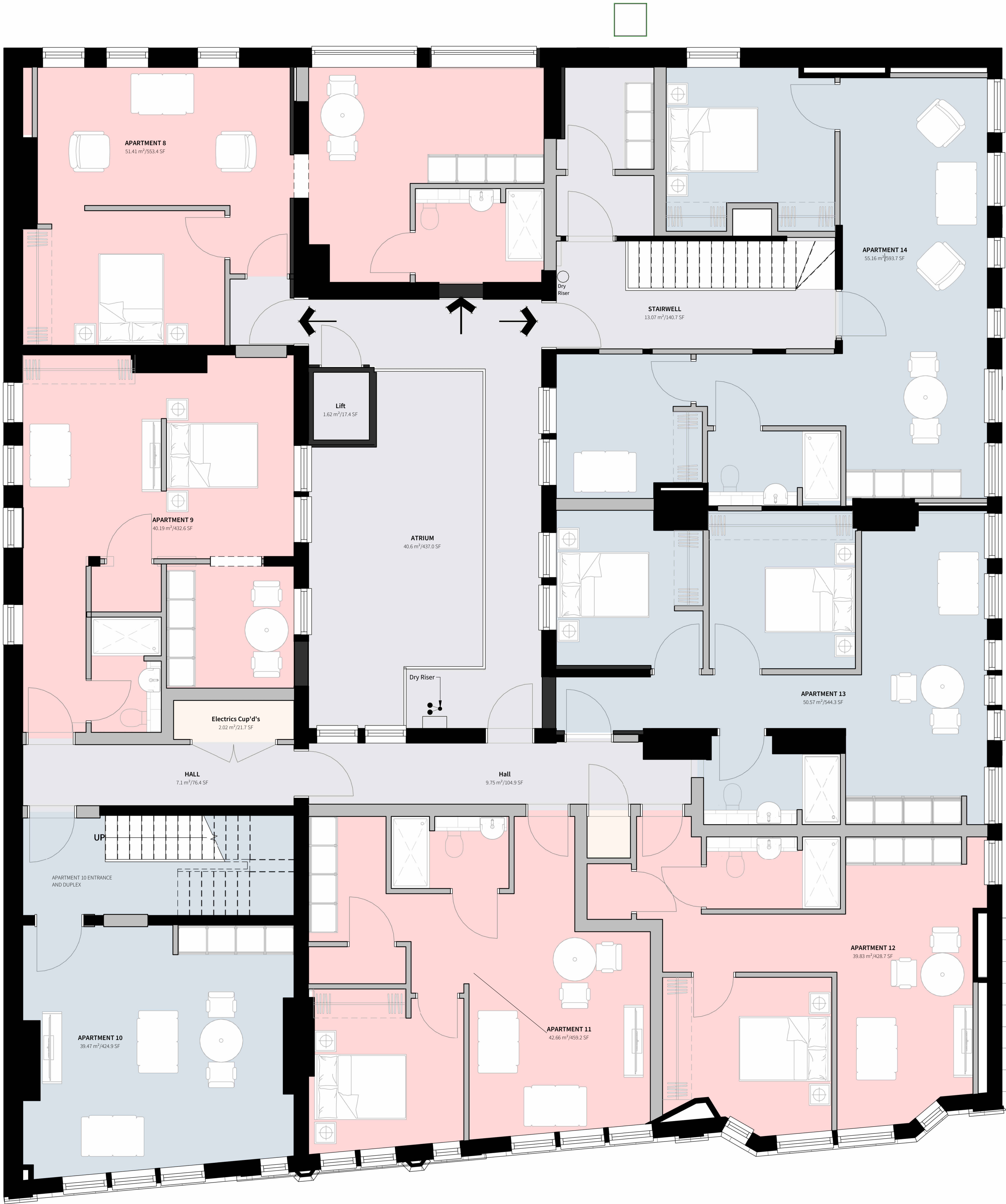
1 PROPOSED - SECOND FLOOR PLAN 1:50
