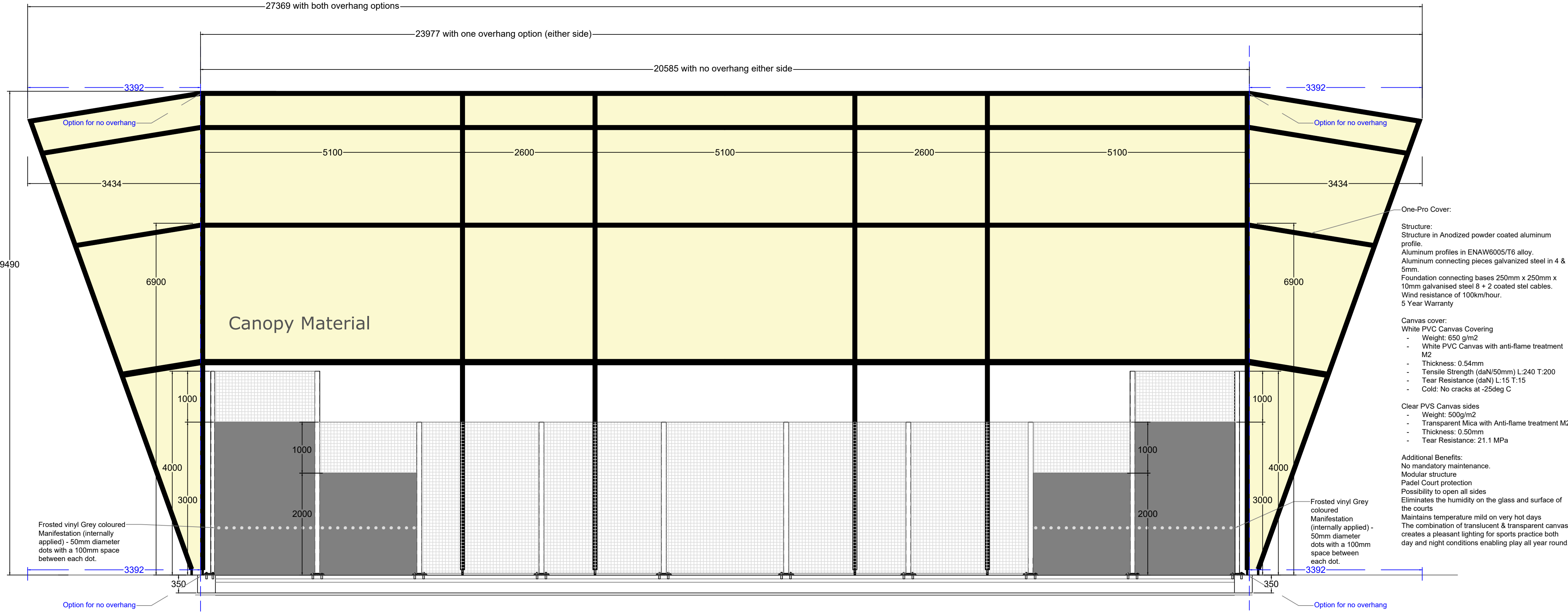
Proposed MejoSet Padel Court with Lusotendas One-Pro Cover - Side Elevation Scale: 1:50@A1
