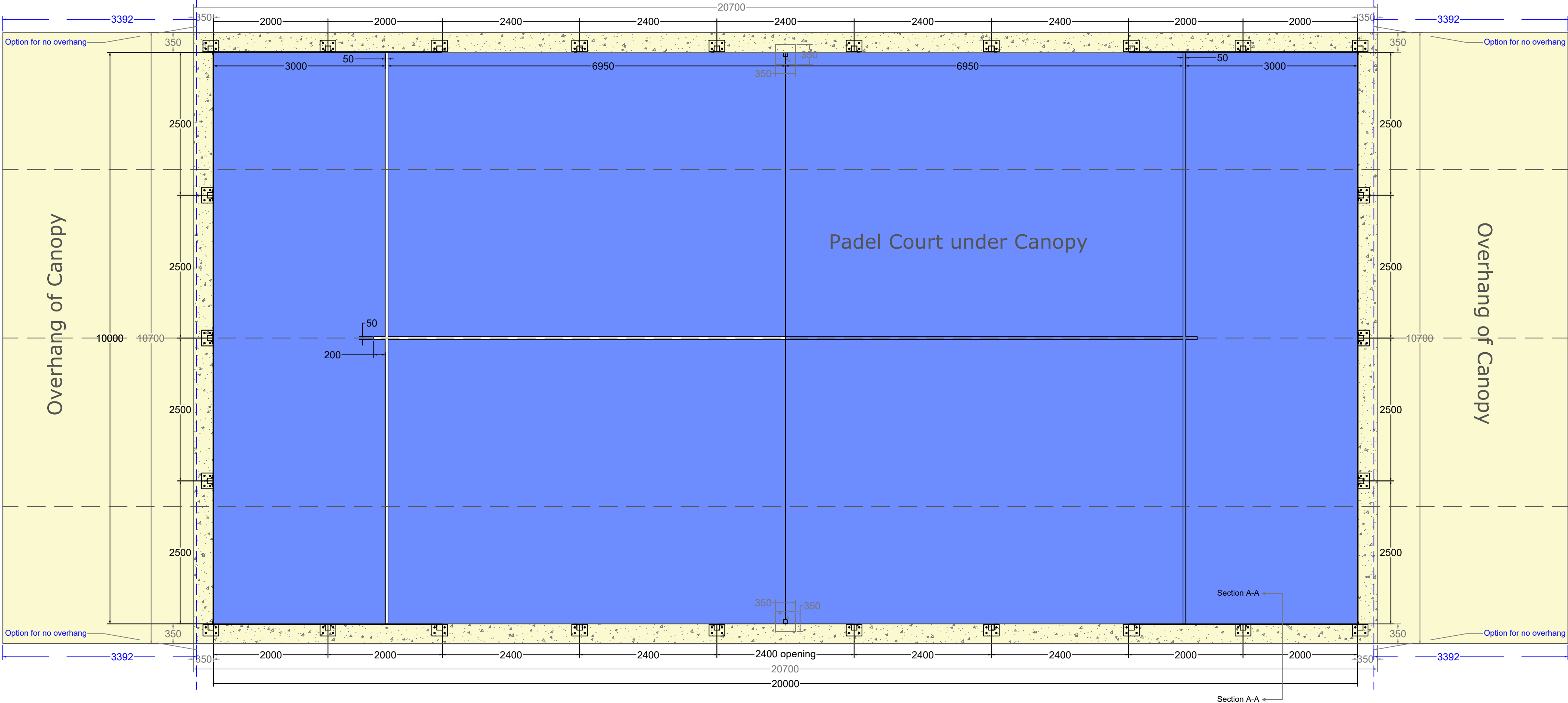
Proposed MejoSet Padel Court with Lusotendas One-Pro Cover - Plan View Scale: 1:50@A1
