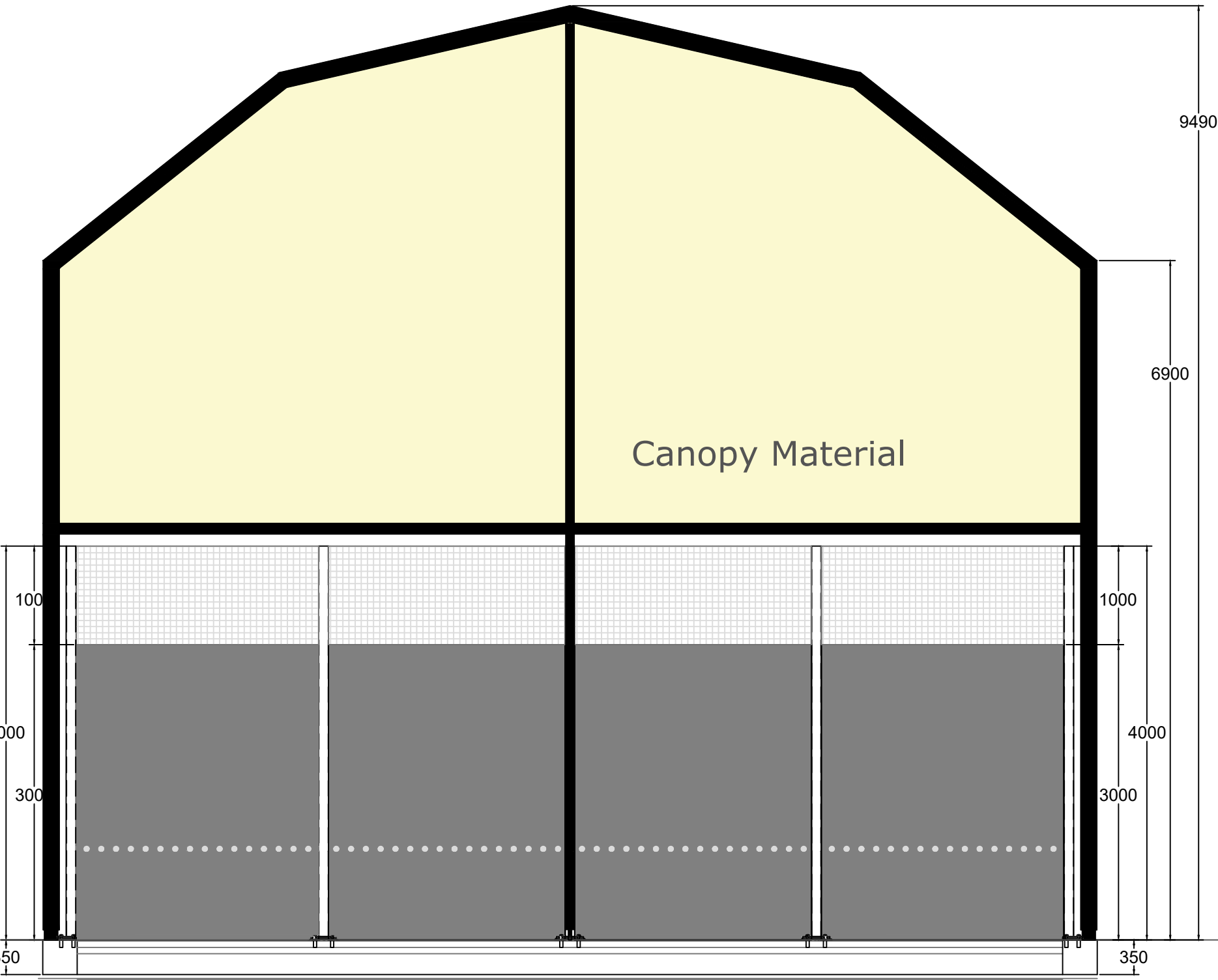
Proposed MejoSet Padel Court with Lusotendas One-Pro Cover - End Elevation Scale: 1:50@A1
