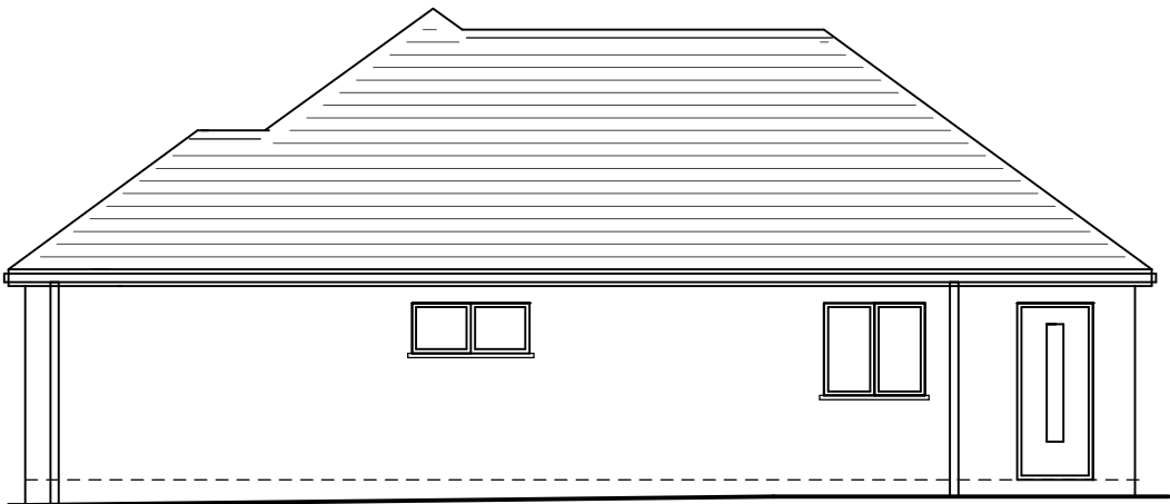
right (south) elevation
