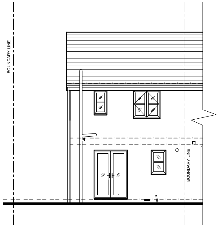
EXISTING REAR
