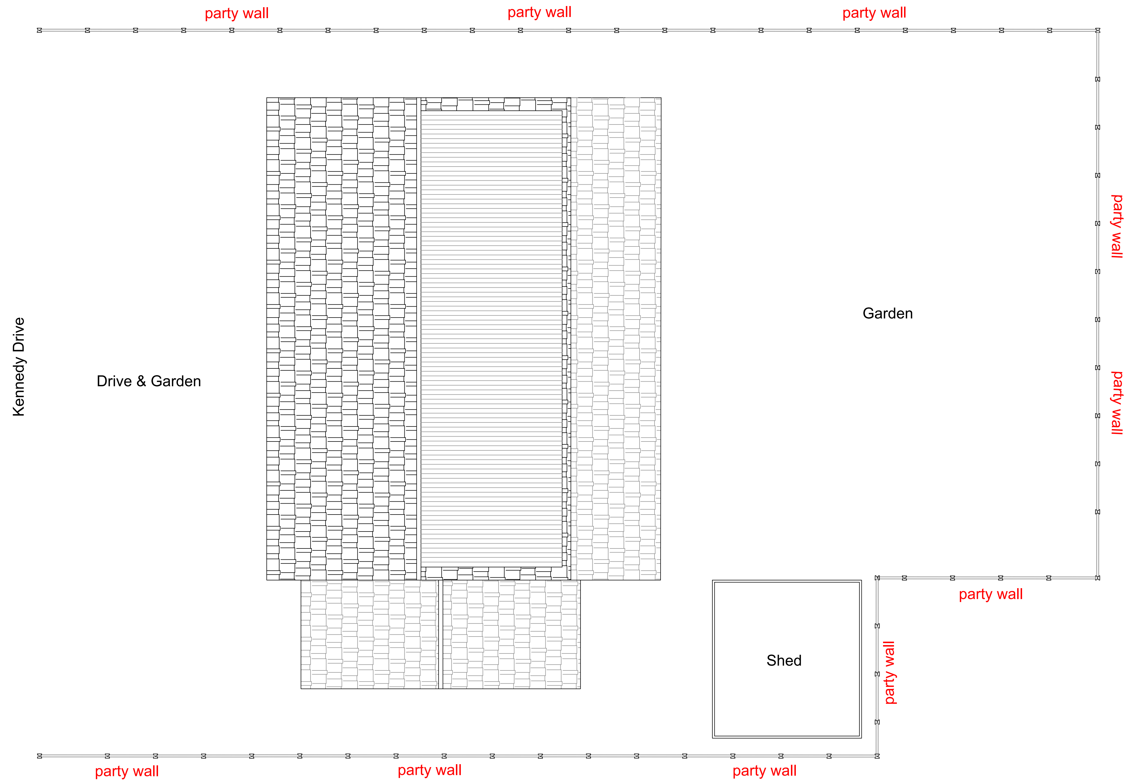
PROPOSED GROUND FLOOR PLAN 1:50 @ A1
