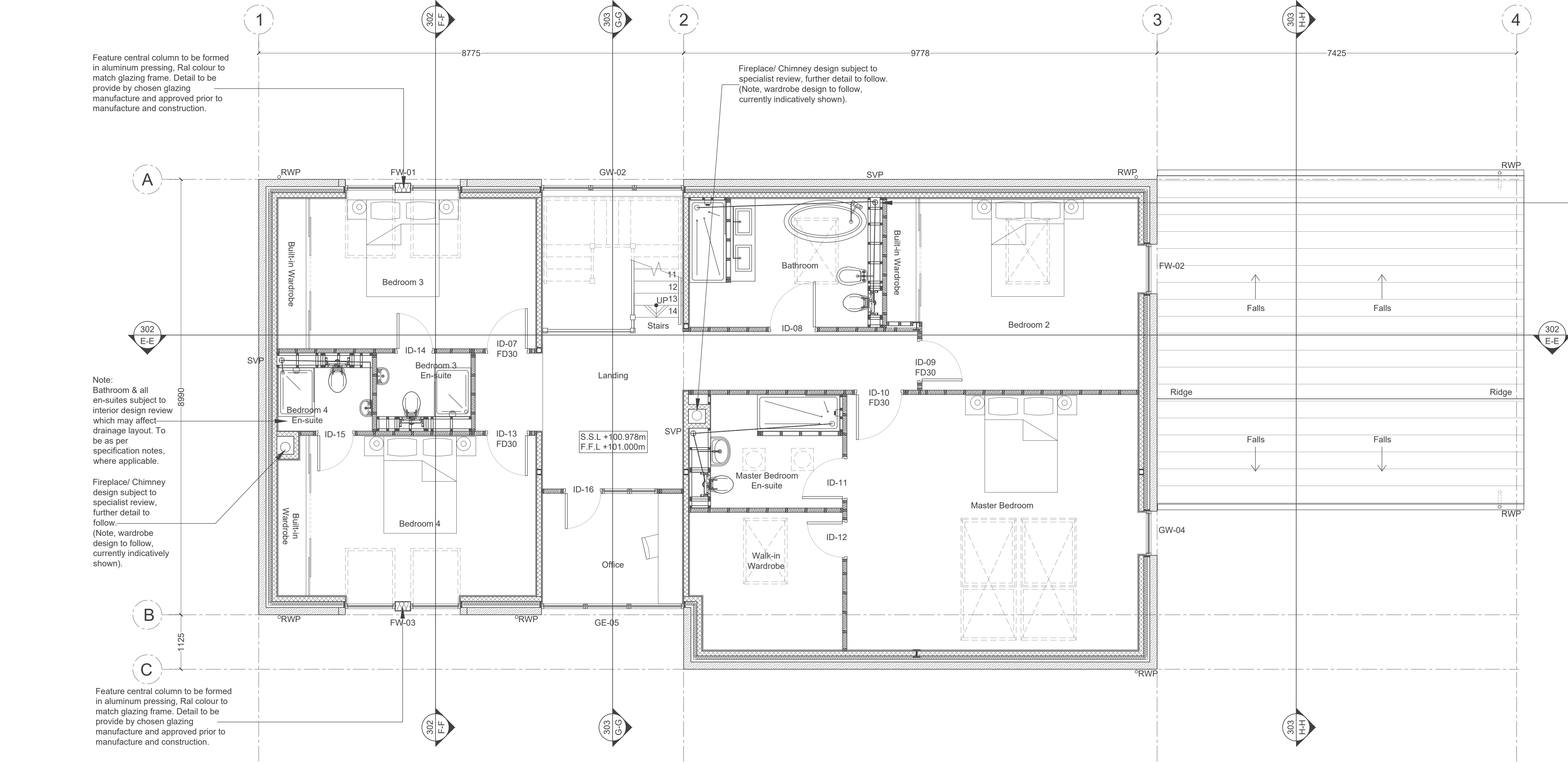
Detached House Proposed First Floor GA Plan Scale 1:50
