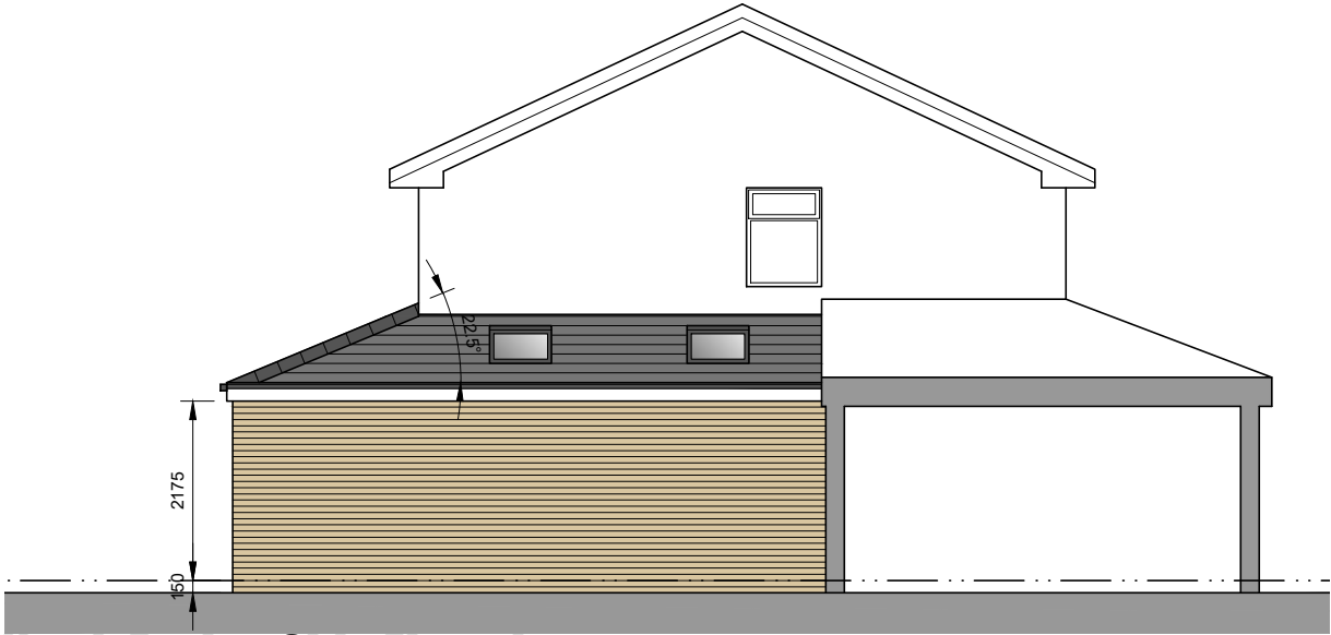
North Facing Side Elevation
