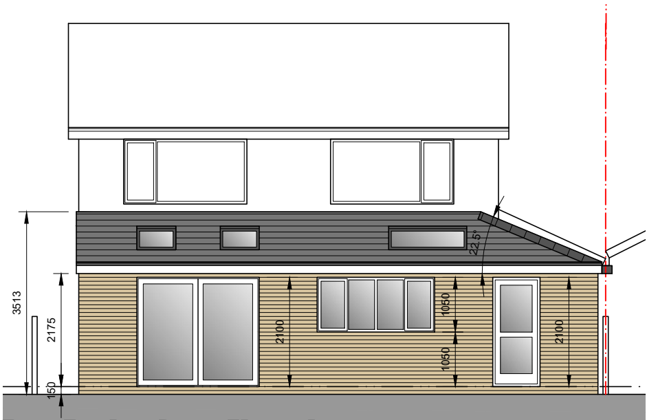
East Facing Rear Elevation
