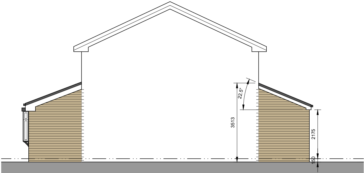
East Facing Side Elevation
