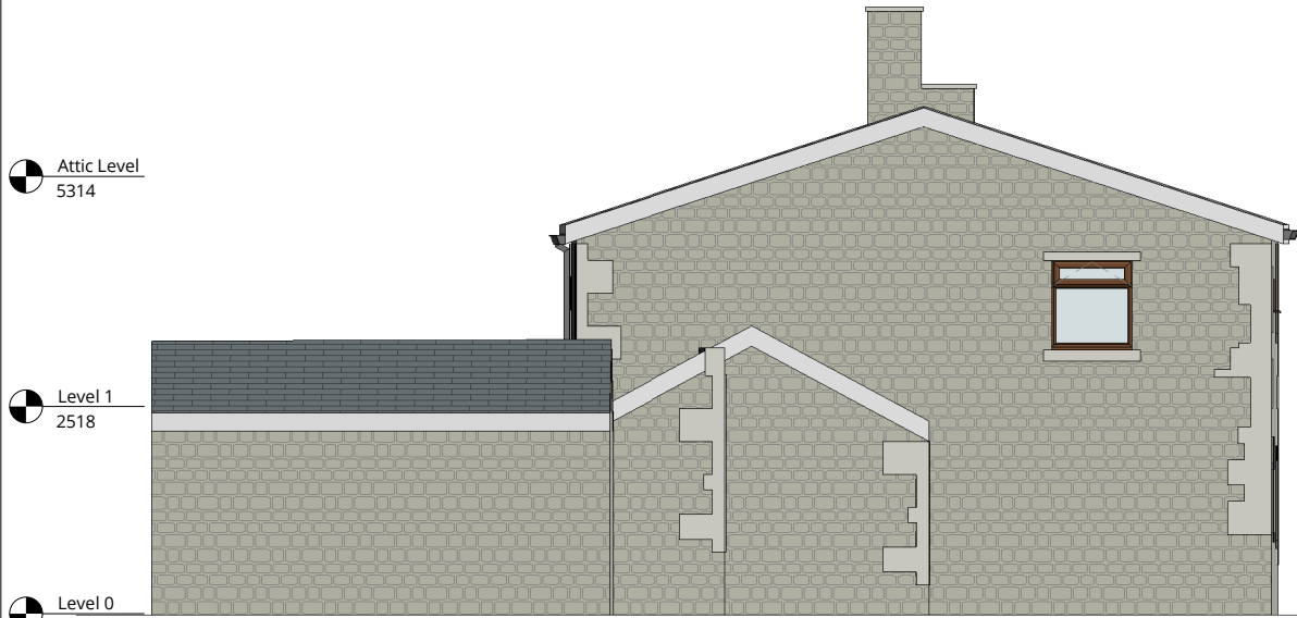
3 Existing South Elevation 1 : 100
