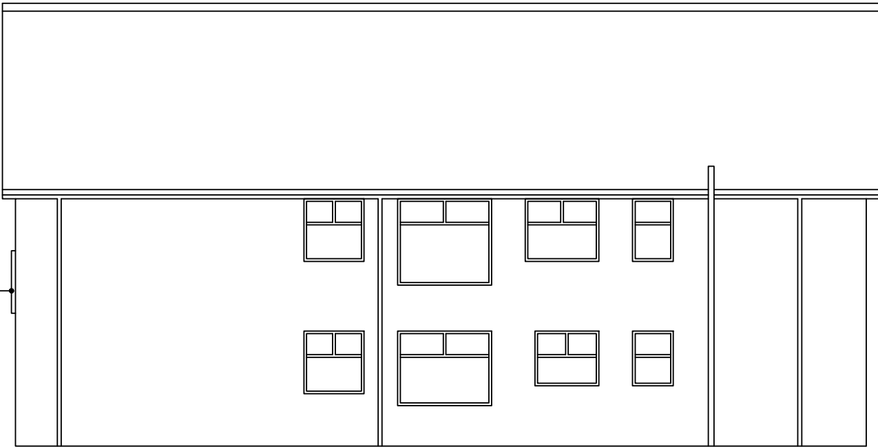
01 Proposed left elevation 1:100
