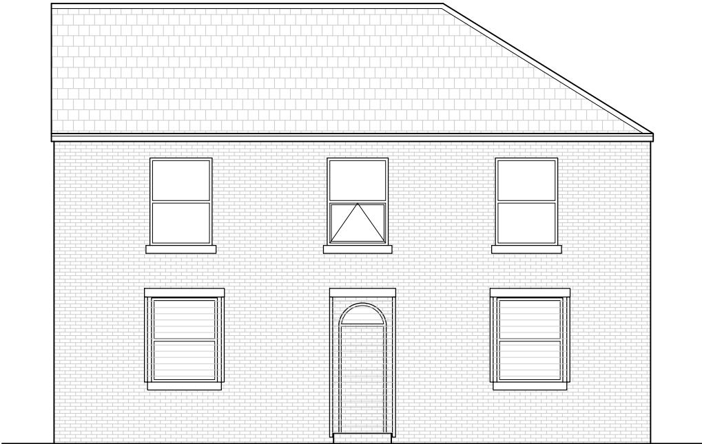
EXISTING FRONT ELEVATION 1:100 @ A3
