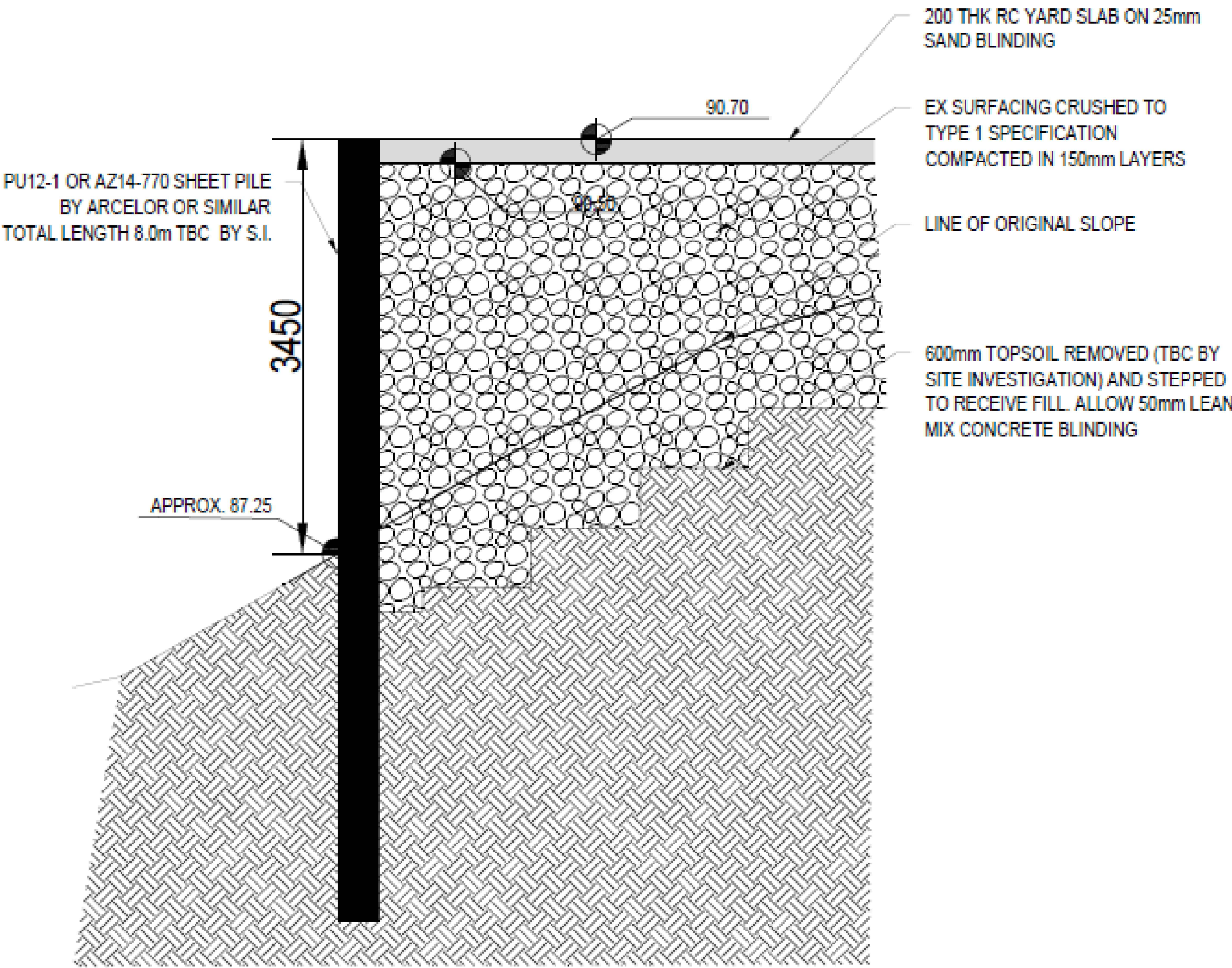
PART SECTION SHOWING MAX RETENTION HEIGHT SCALE 1:50
