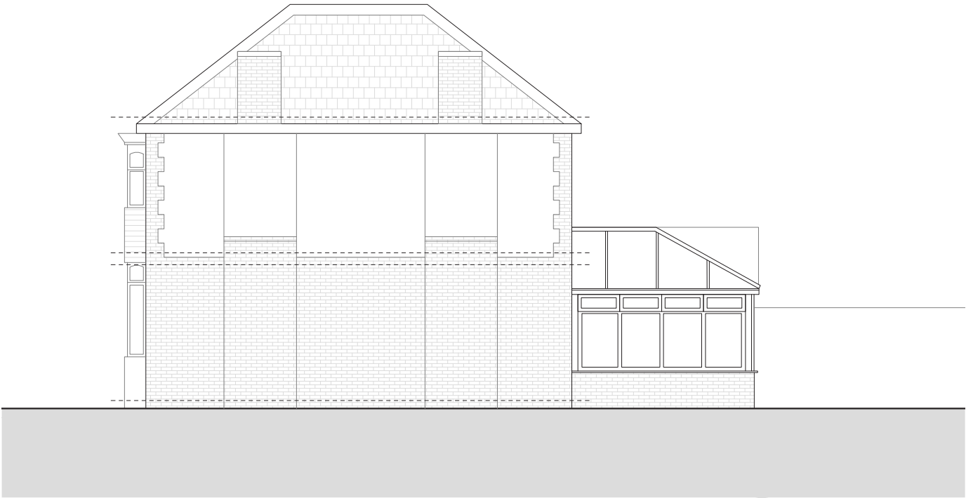
EXISTING SIDE ELEVATION FROM 2 CRAIGWELL ROAD 1:100 @ A3
