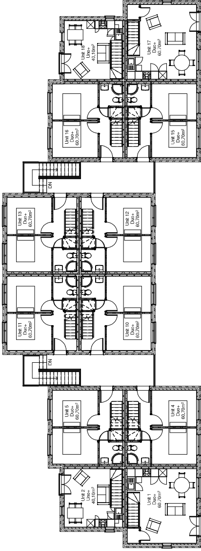
2 Proposed First Floor Plan 1 : 100
